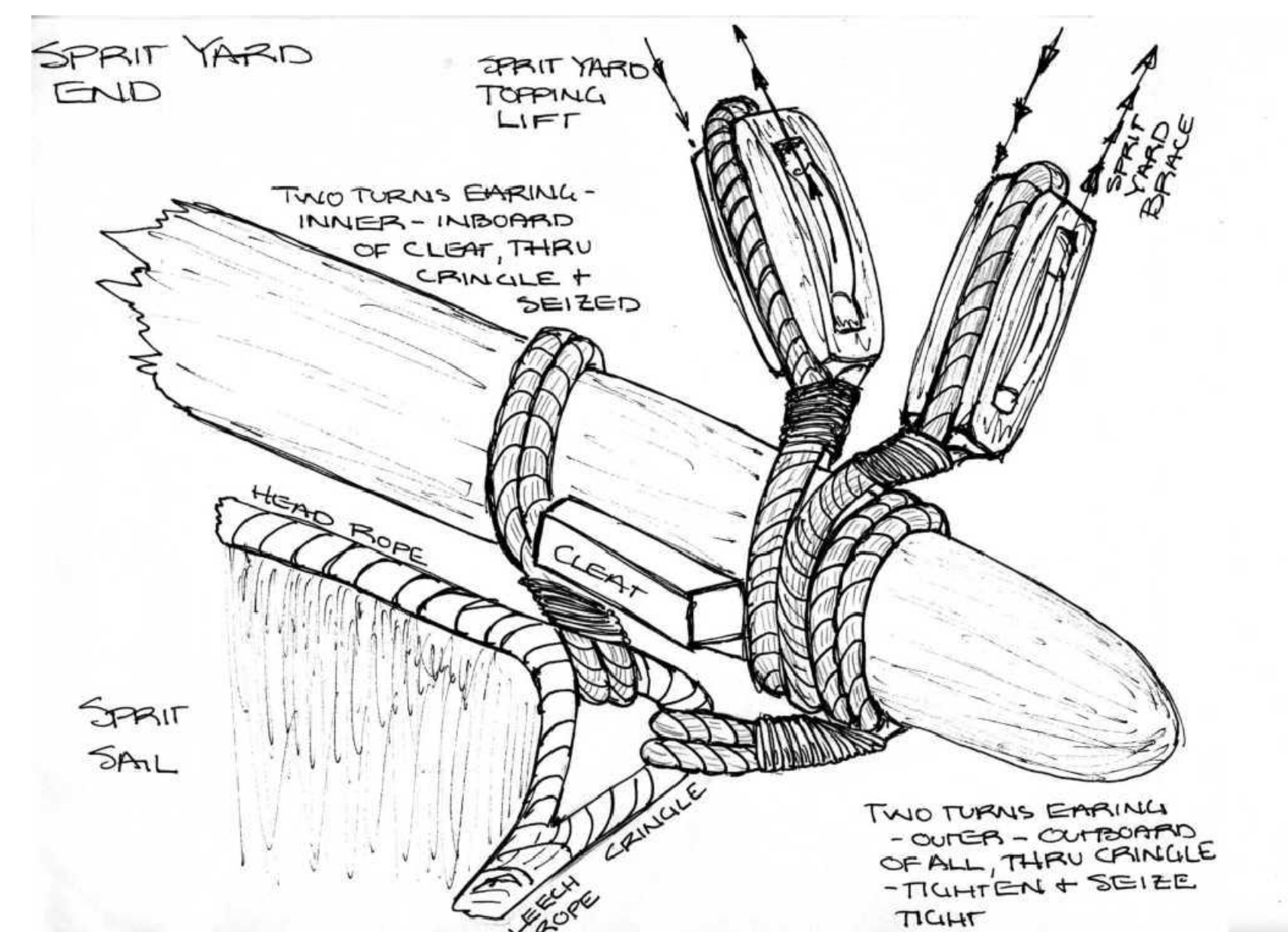
DETAIL: B-44 SPRITSAIL YARD OUTBOARD ENDS ARRANGEMENT NO SCALE
