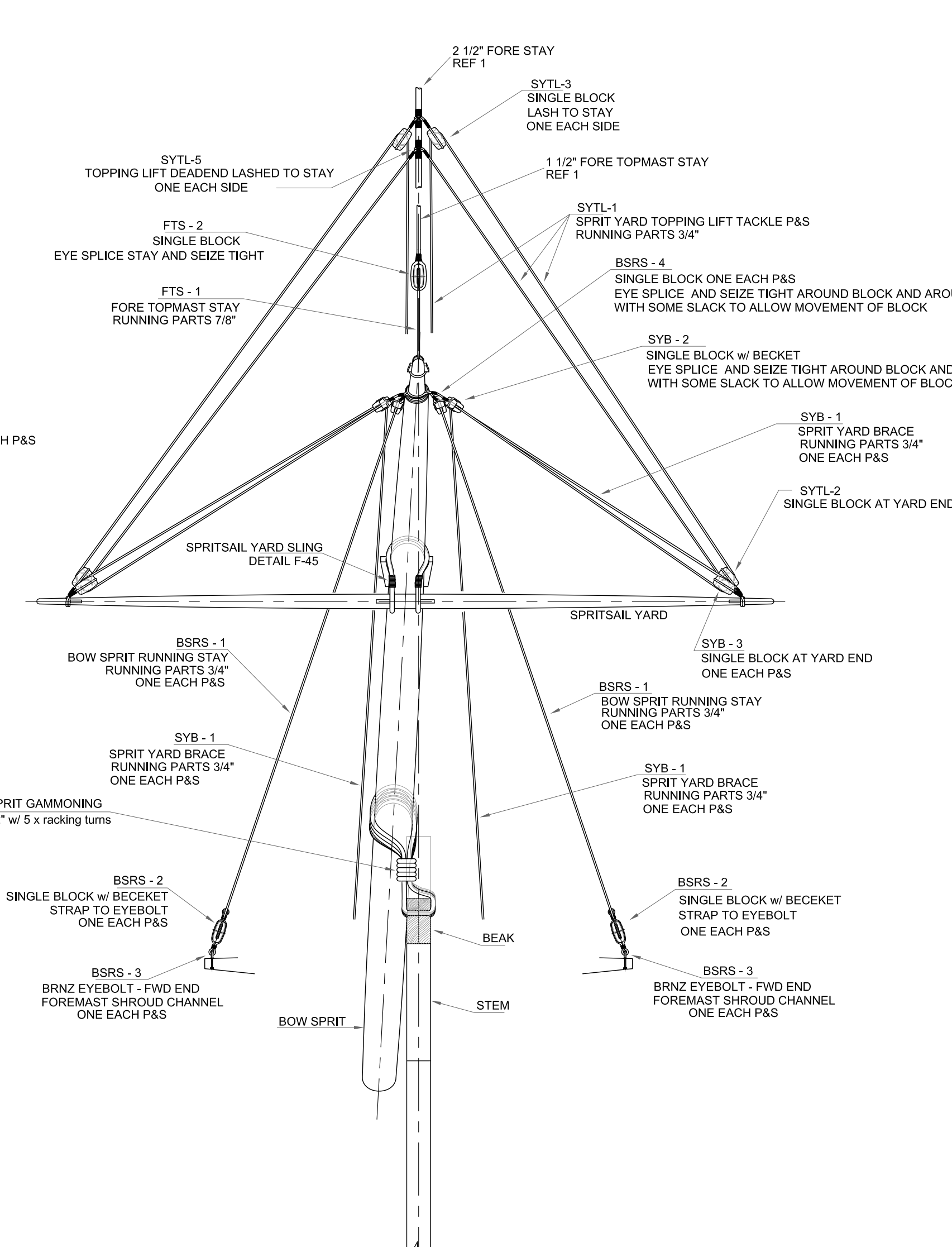
DETAIL: G-44 BOWSPRIT LOOKING AFT FROM AHEAD SCALE: 1/4" = 1'-0"
