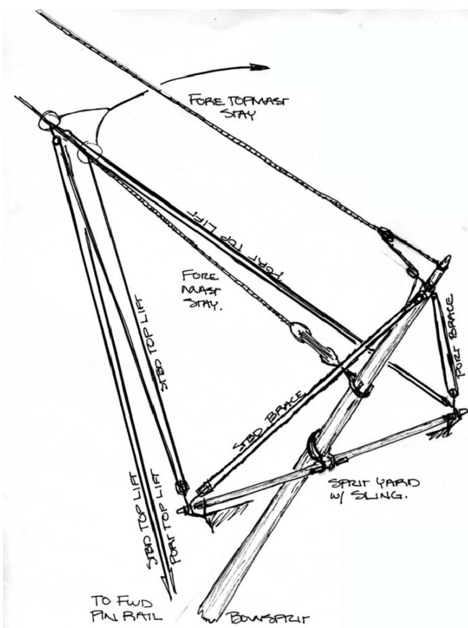
DETAIL: B-47 SPRITSAIL YARD LIFT AND BRACE ARRANGEMENT SKETCH NO SCALE
