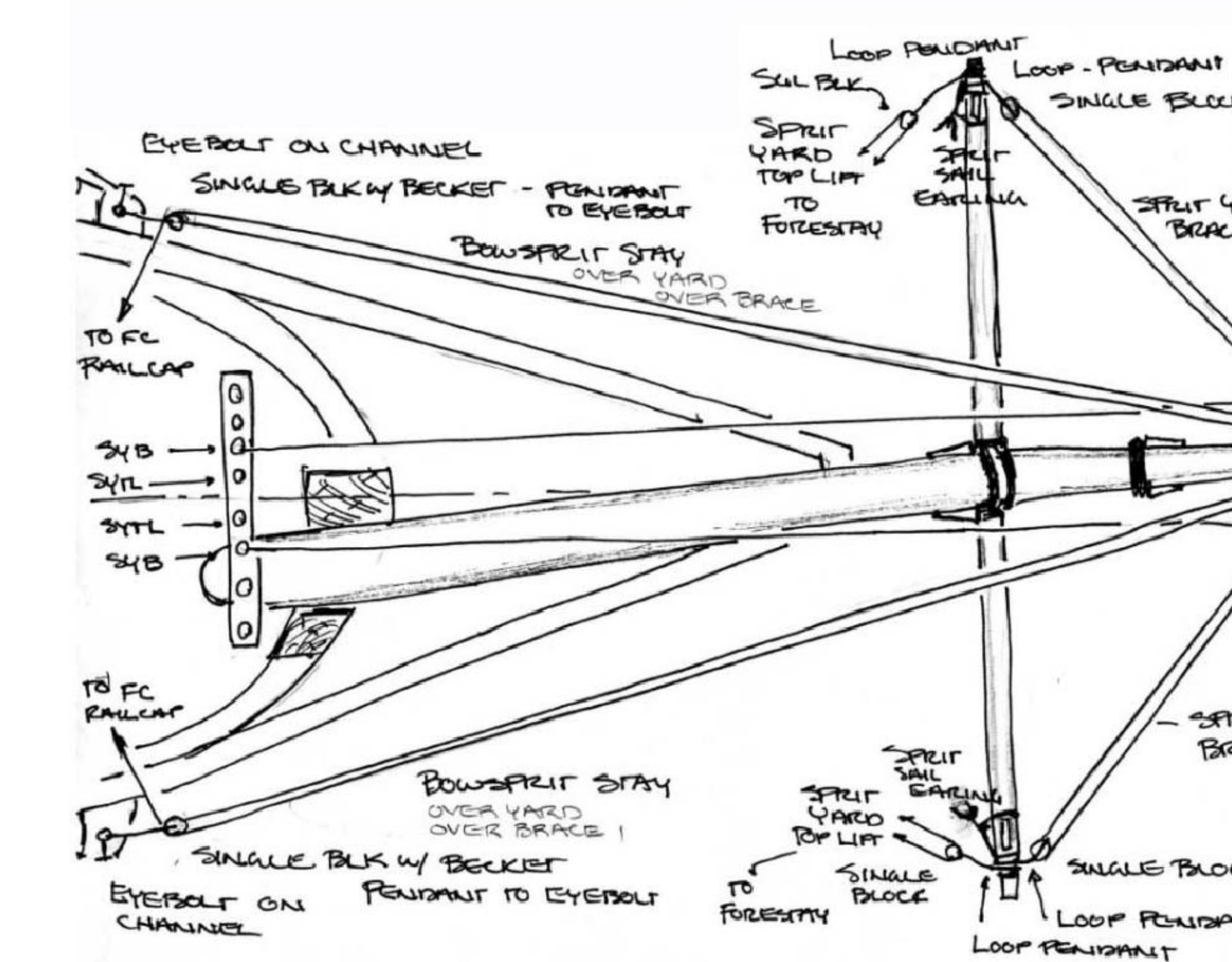
DETAIL: E-46 BOWSPRIT AND SPRITSAIL YARD PLAN ARRANGEMENT SKETCH NO SCALE
