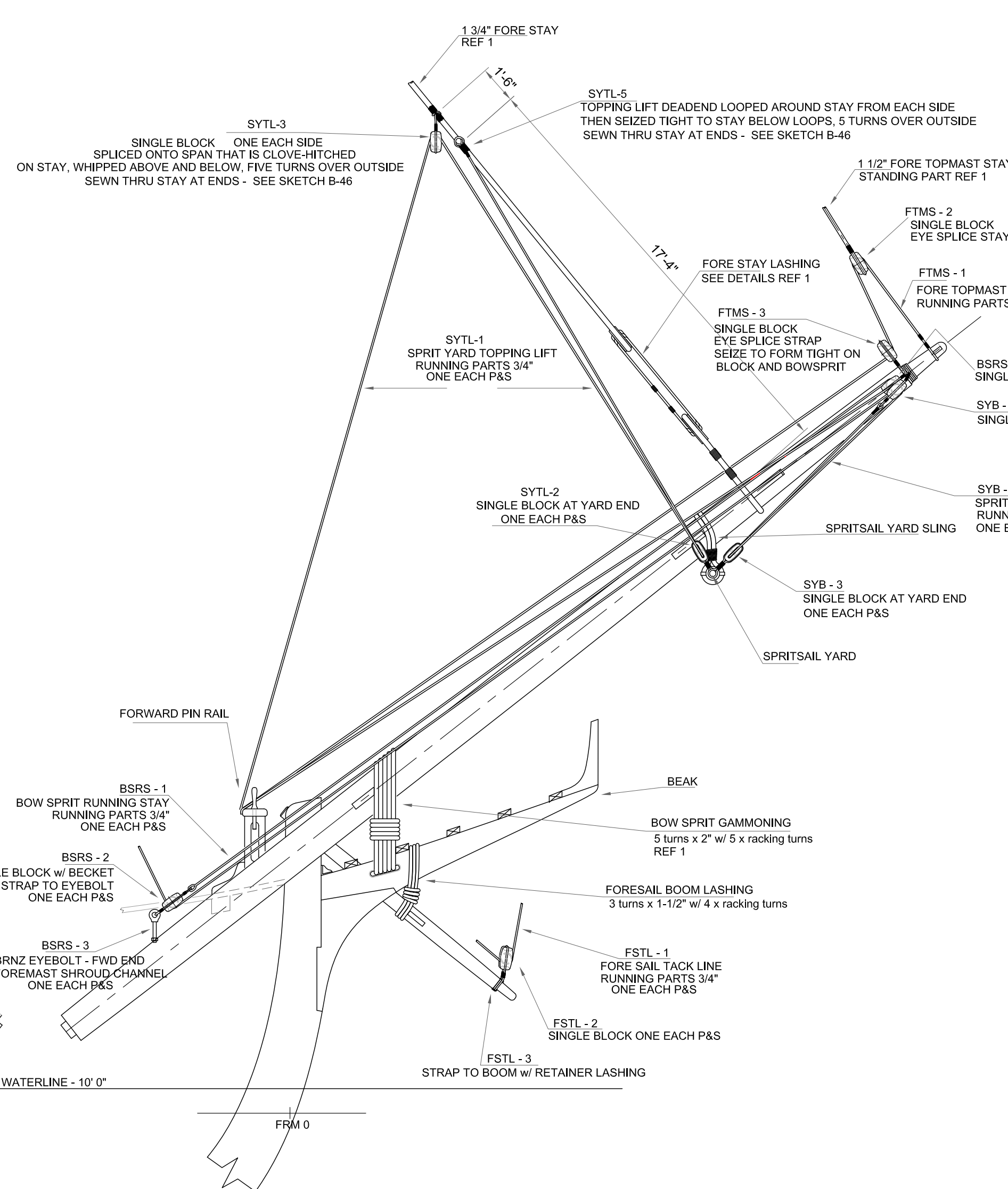
DETAIL: G-46 BOWSPRIT AND FORESAIL BOOM - STBD SIDE SCALE: 1/4" = 1'-0"
