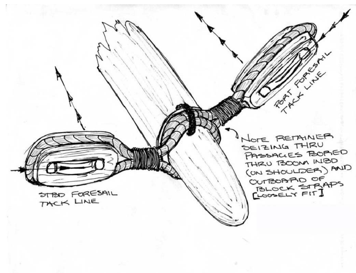
DETAIL: F-48 END OF FORESAIL BOOM ARRANGEMENT NO SCALE
