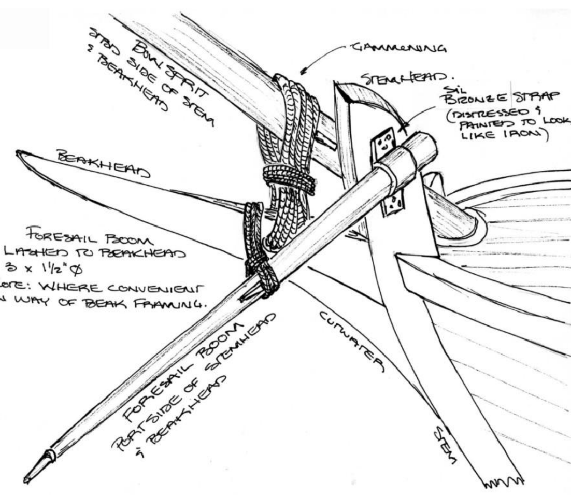
DETAIL: B-42 BOWSPRIT AND FORESAIL BOOM - PORT SIDE NO SCALE
