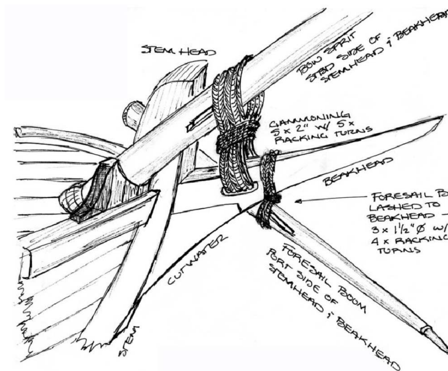
DETAIL: F-42 BOWSPRIT AND FORESAIL BOOM - STBD SIDE NO SCALE
