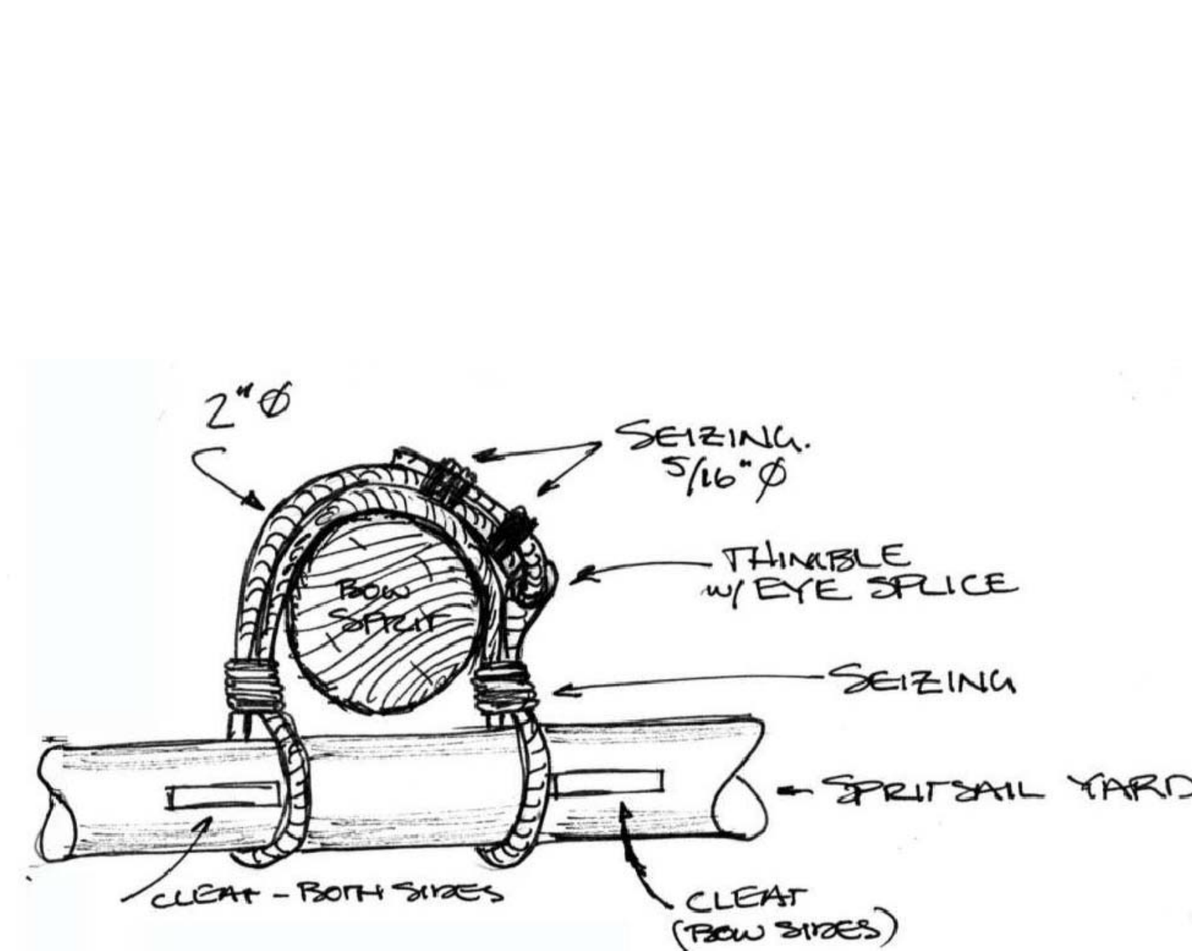
DETAIL: G-44 BOWSPRIT LOOKING AFT FROM AHEAD SCALE: 1/4" = 1'-0"
