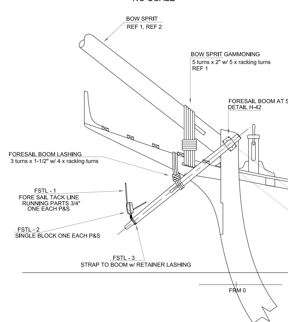
DETAIL: G-48 BOWSPRIT AND FORESAIL BOOM - PORT SIDE SCALE: 1/4" = 1'-0"
