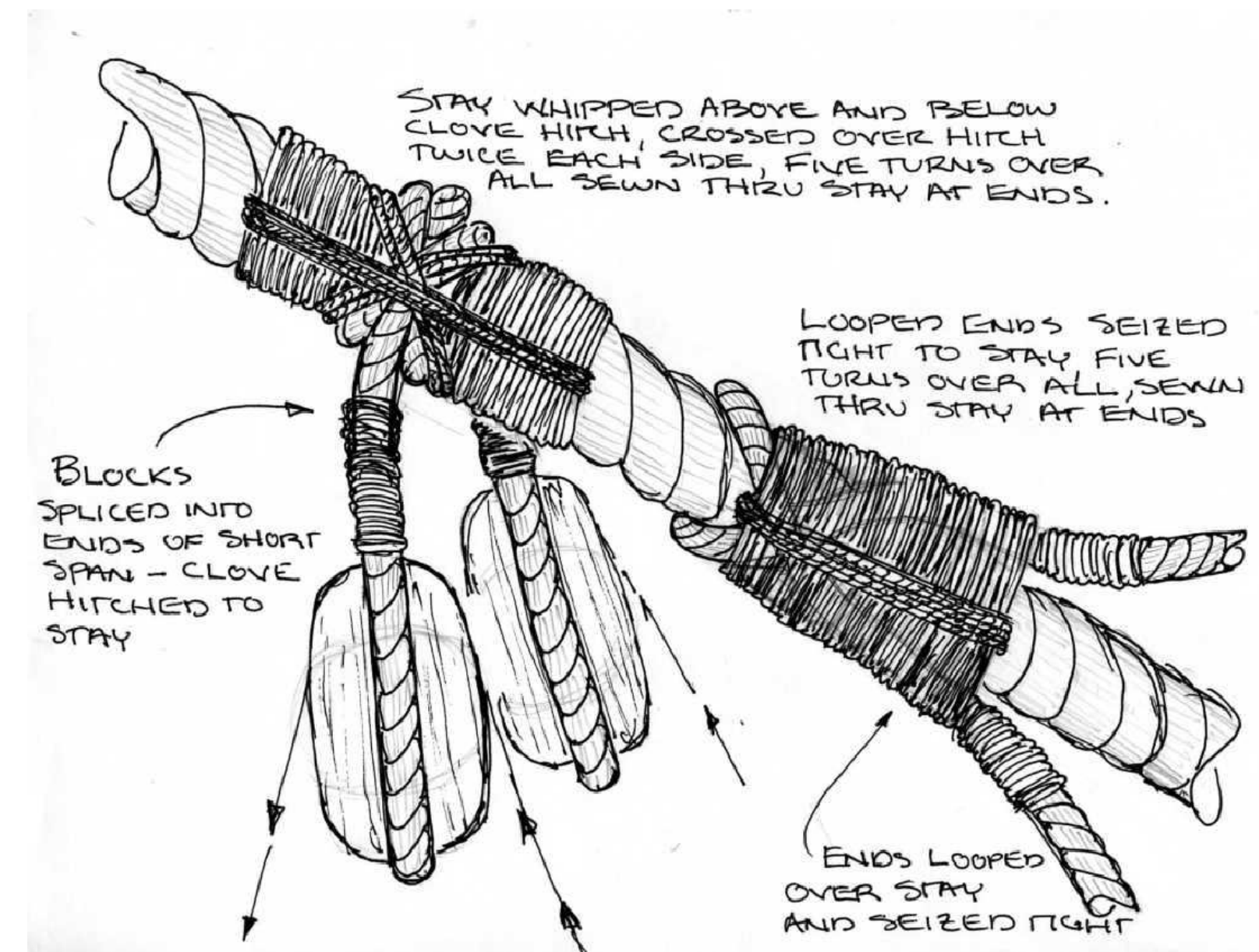
DETAIL: B-46 SPRITSAIL YARD TOPPING LIFT ATTACHMENT AT FORESTAY NO SCALE
