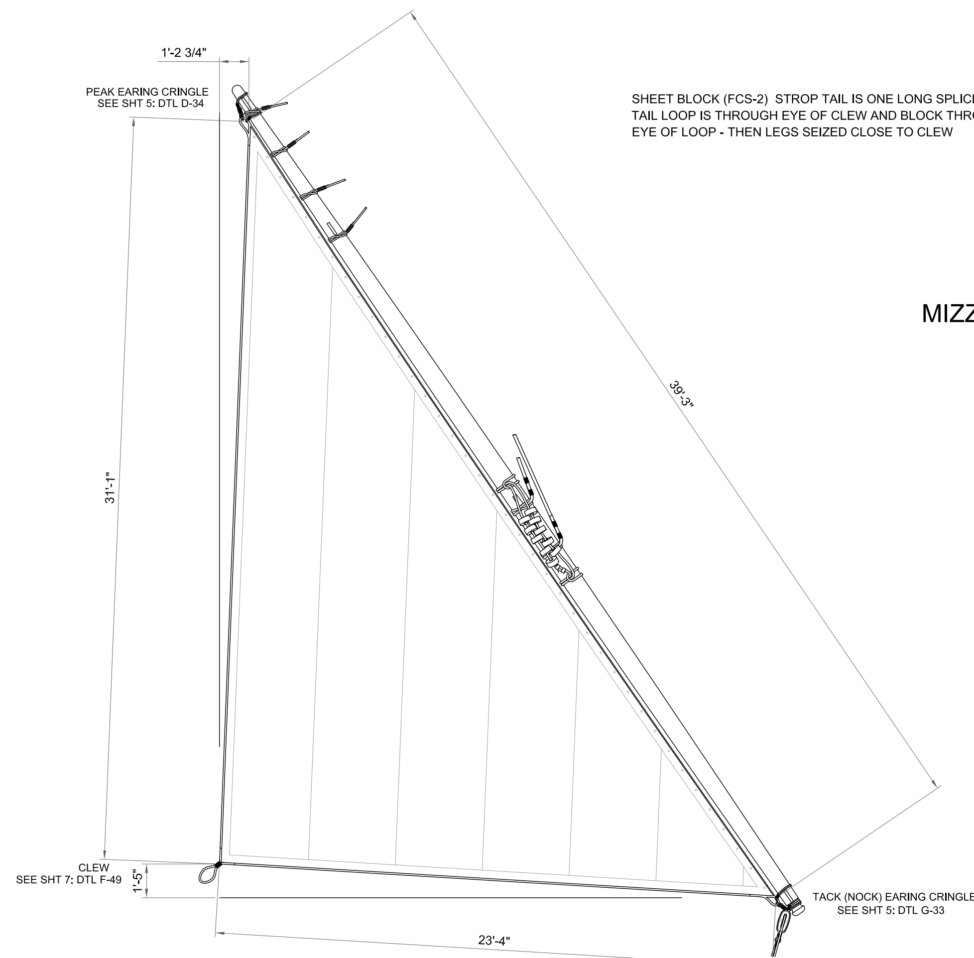
DETAIL: D-50 LATEEN MIZZEN SAIL SCALE: 1/4" = 1'-0"
