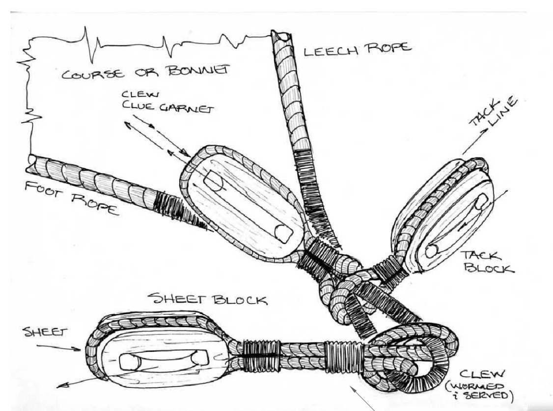
DETAIL: A-56 MAIN COURSE OR BONNET BLOCKS AT CLEW NOT TO SCALE
