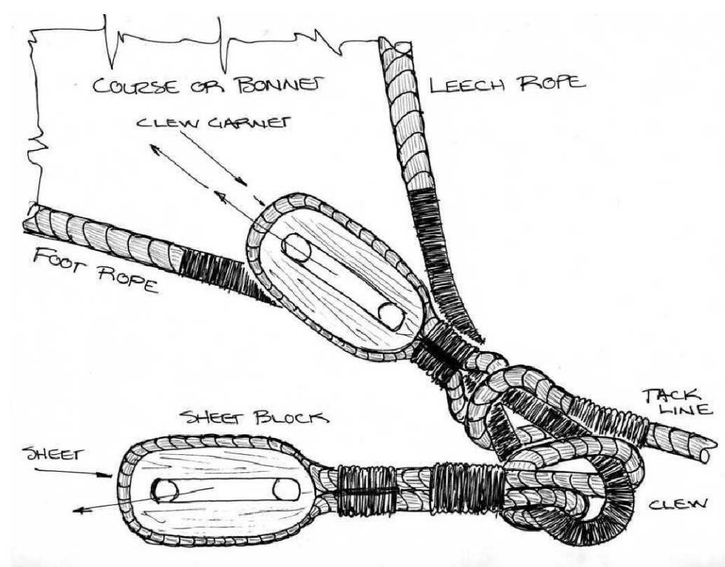
DETAIL: A-54 FORE COURSE OR BONNET BLOCKS AT CLEW NOT TO SCALE
