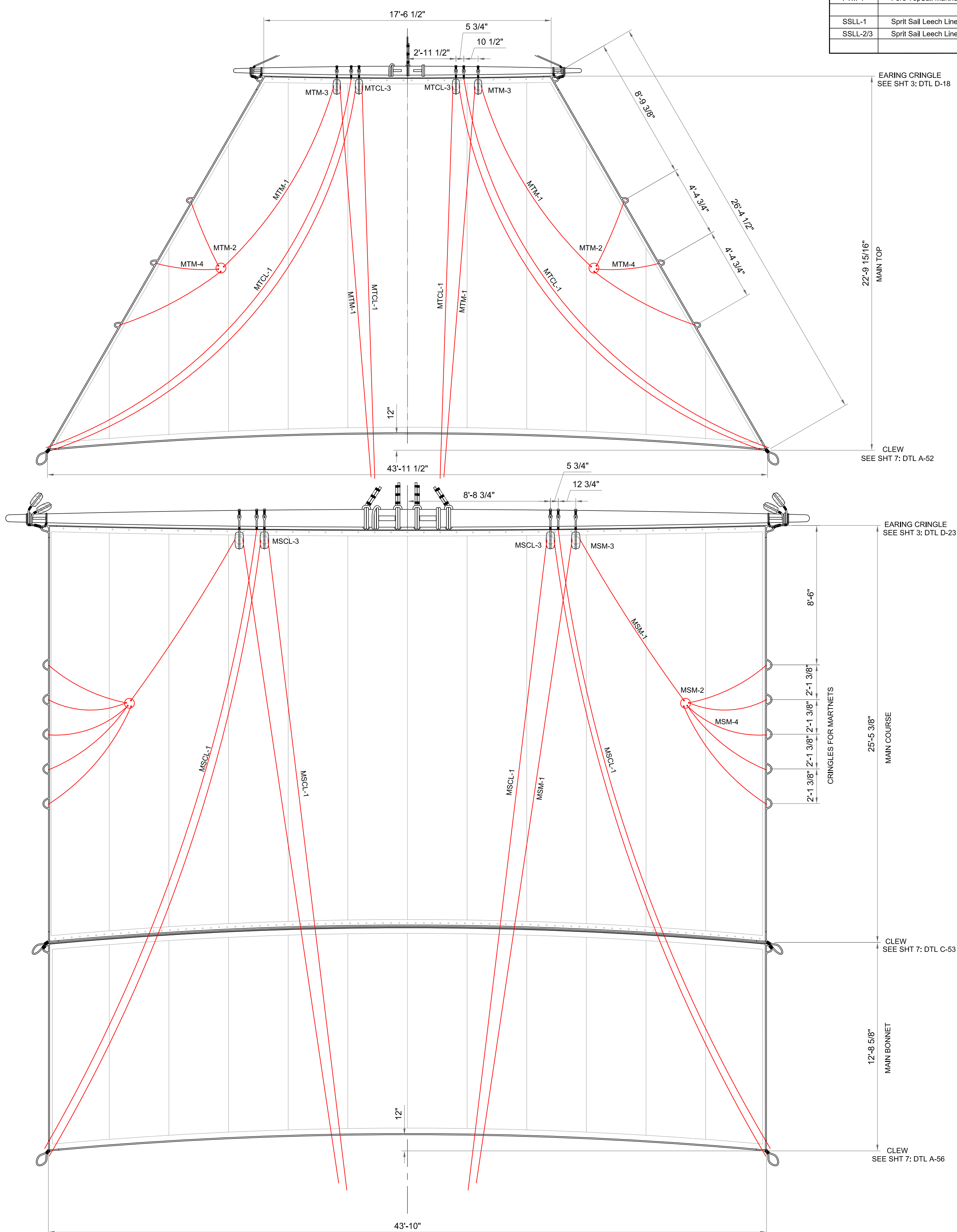
DETAIL: E-55 MAIN MAST SAILS SCALE: 1/4" = 1'-0"
