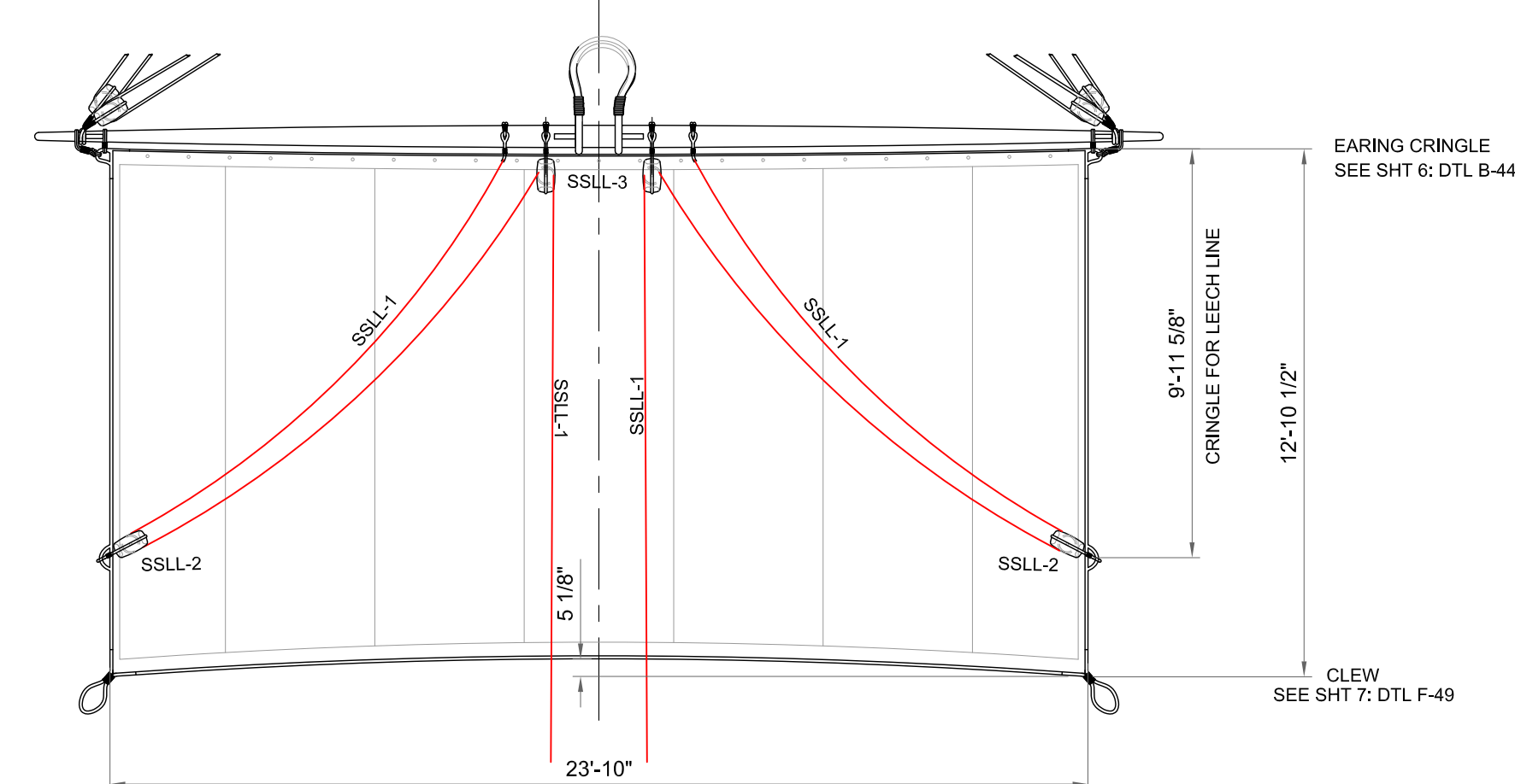
DETAIL: H-50 SPRIT SAIL SCALE: 1/4" = 1'-0"
