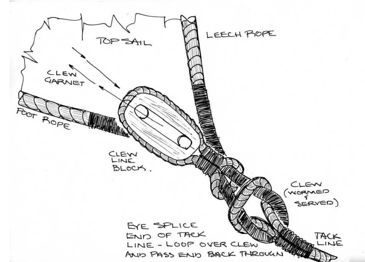
DETAIL: A-52 TYPICAL TOP SAIL CLEW ARRANGEMENT NOT TO SCALE
