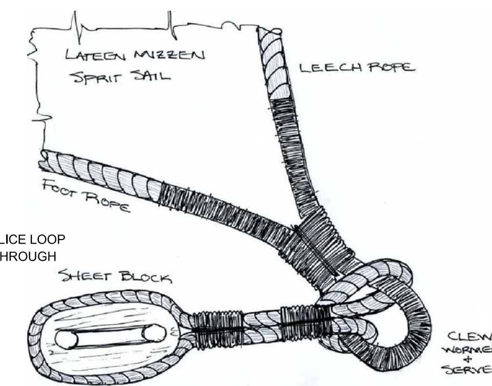
DETAIL: F-49 MIZZEN AND SPRIT SAILS CLEW ARRANGEMENT NOT TO SCALE
