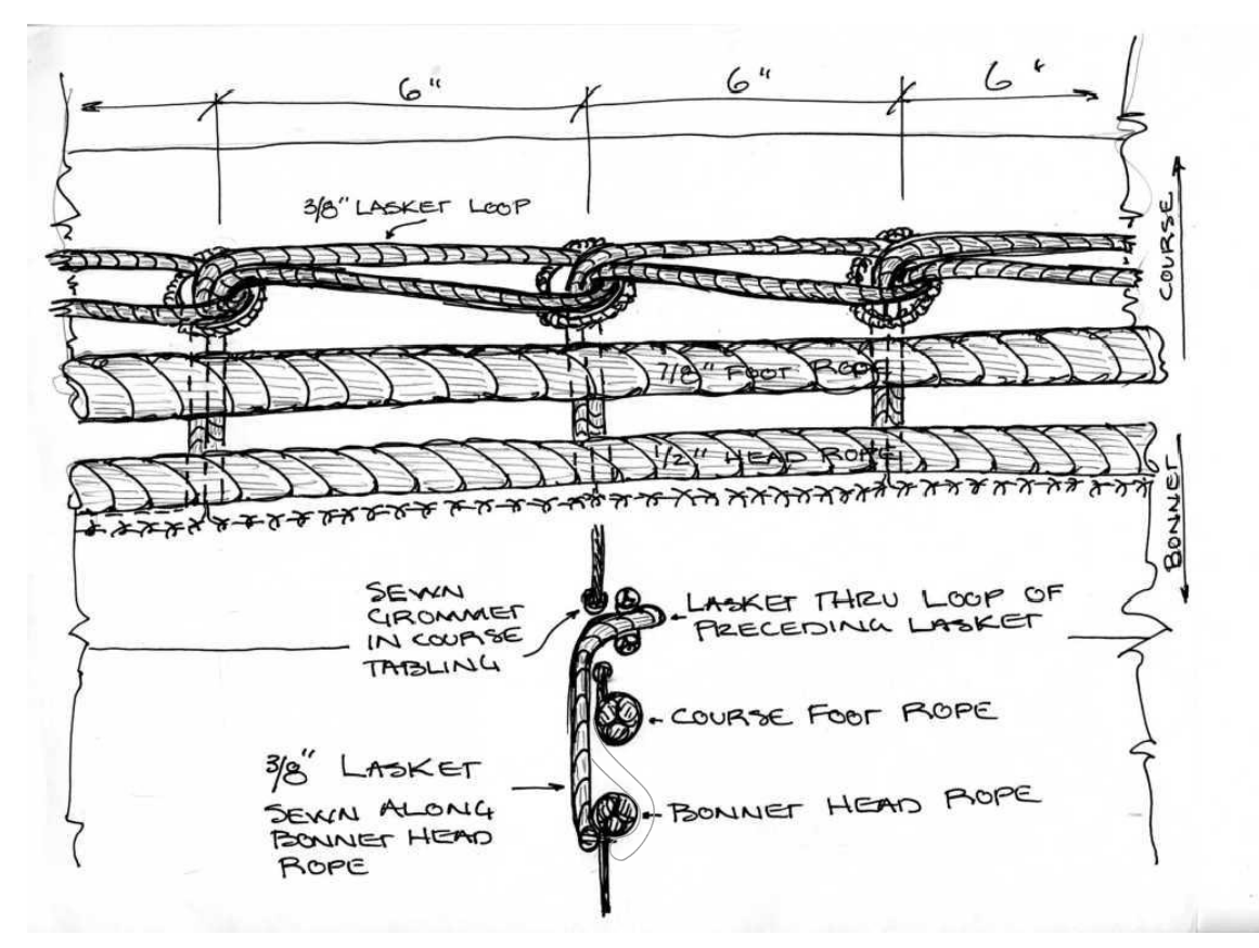
DETAIL: C-54 TYPICAL BONNET TO COURSE ATTACHMENT 3/8" CONTINUOUS SEWN IN APPROX 12" LASKETS (LOOPS) note: stagger sewn legs of lasket on opposite sides of bonnet headrope NOT TO SCALE
