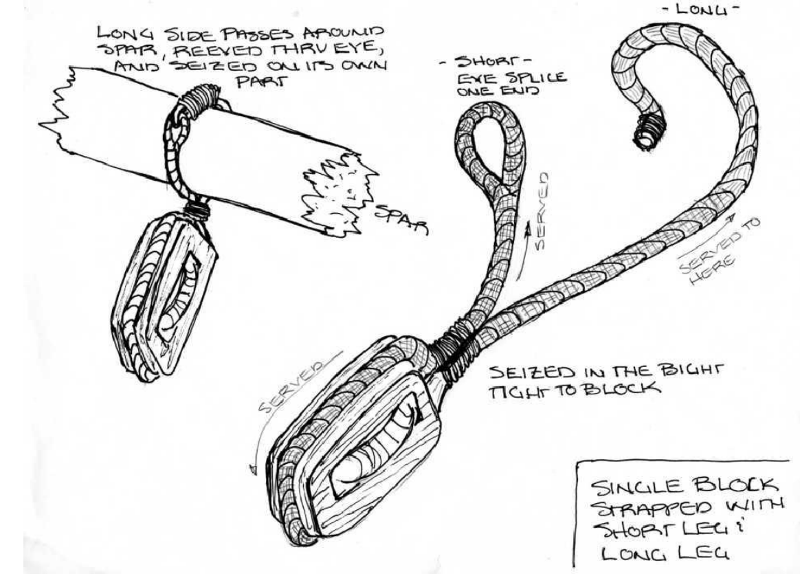
DETAIL: A-50 TYPICAL SINGLE BLOCK ATTACHMENT AT YARD PER CLEW GARNET AND LEECH LINE BLOCKS NOT TO SCALE
