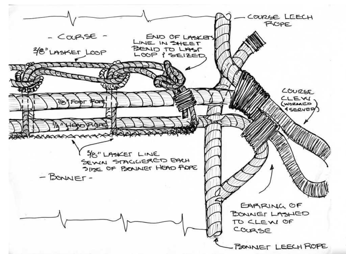
DETAIL: C-53 TYPICAL BONNET TO COURSE ATTACHMENT AT OUTBOARD ENDS NOT TO SCALE
