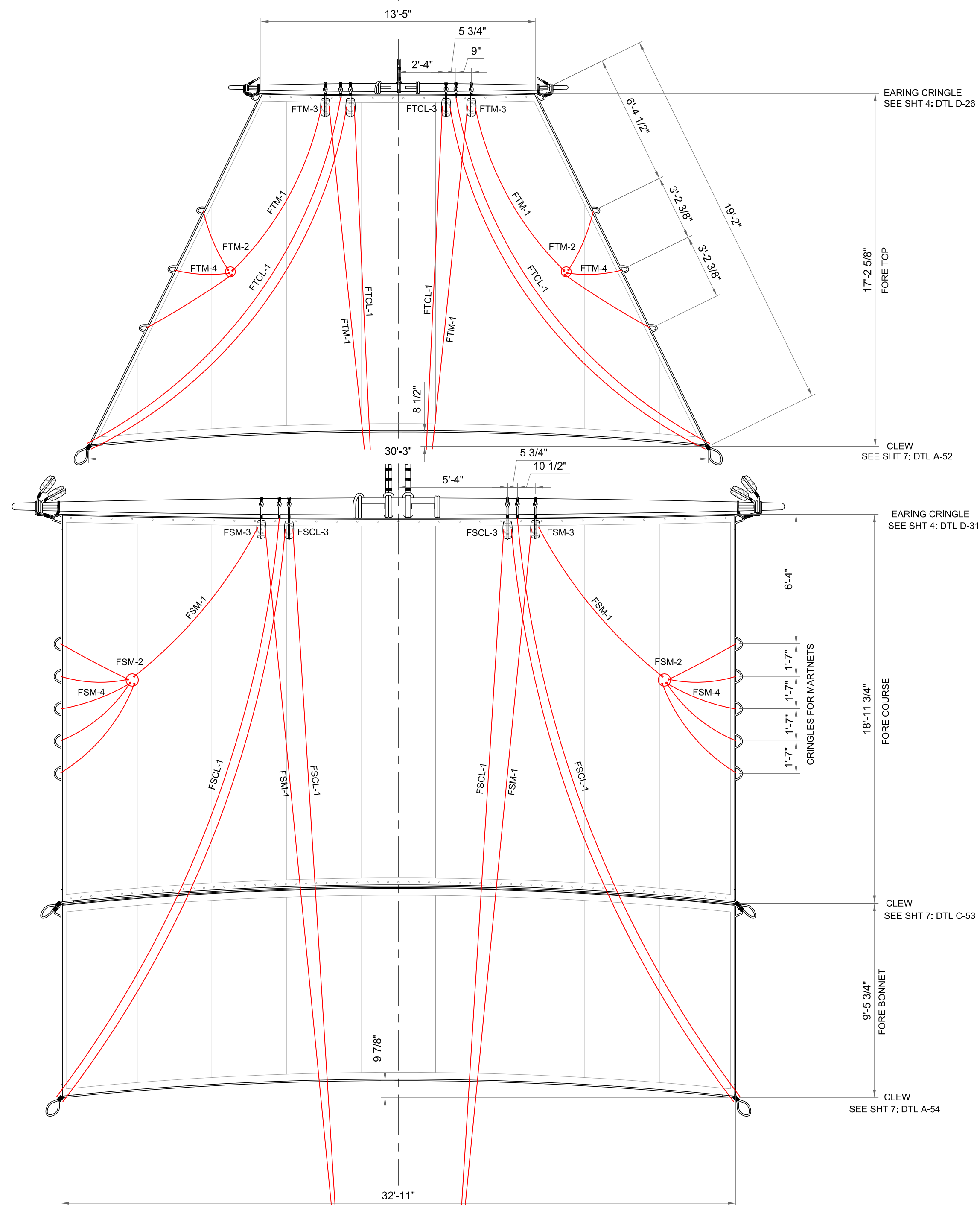
DETAIL: E-53 FORE MAST SAILS SCALE: 1/4" = 1'-0"
