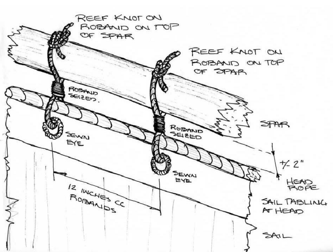
DETAIL: C-56 TYPICAL SAIL ATTACHMENT TO SPAR 5/8" 4 STRAND HEMPEX ROBANDS TYPICAL NOT TO SCALE
