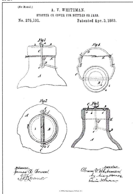
Figure 9 – A.V. Whiteman’s first 1883 patent (U.S. Patent Office)
