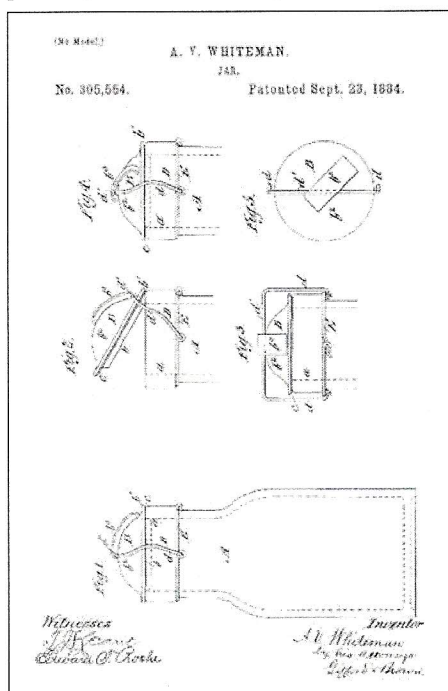
Figure 13 – A.V. Whiteman's 1884 patent (U.S. Patent Office)
