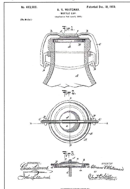
Figure 24 – Whiteman’s 1890 patent (U.S. Patent Office)
