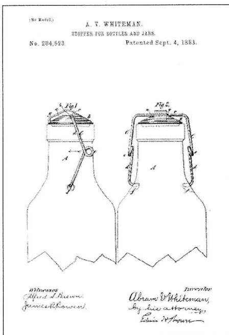
Figure 12 – A.V. Whiteman's second 1883 patent (U.S. Patent Office)
