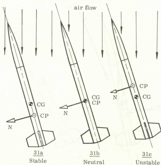
Types of stability
