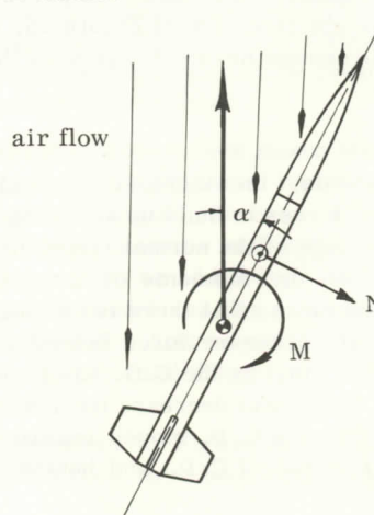
Aerodynamic Moment (unstable condition)
