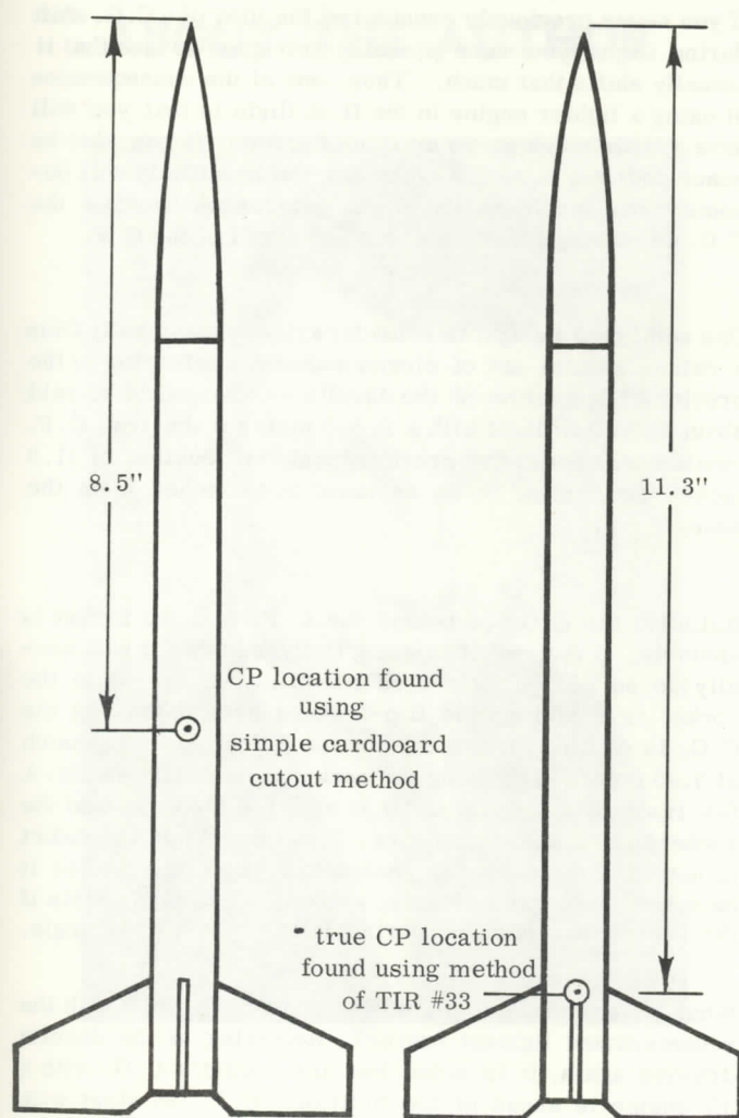
CP locations for Centuri's four-finned JAVELIN
