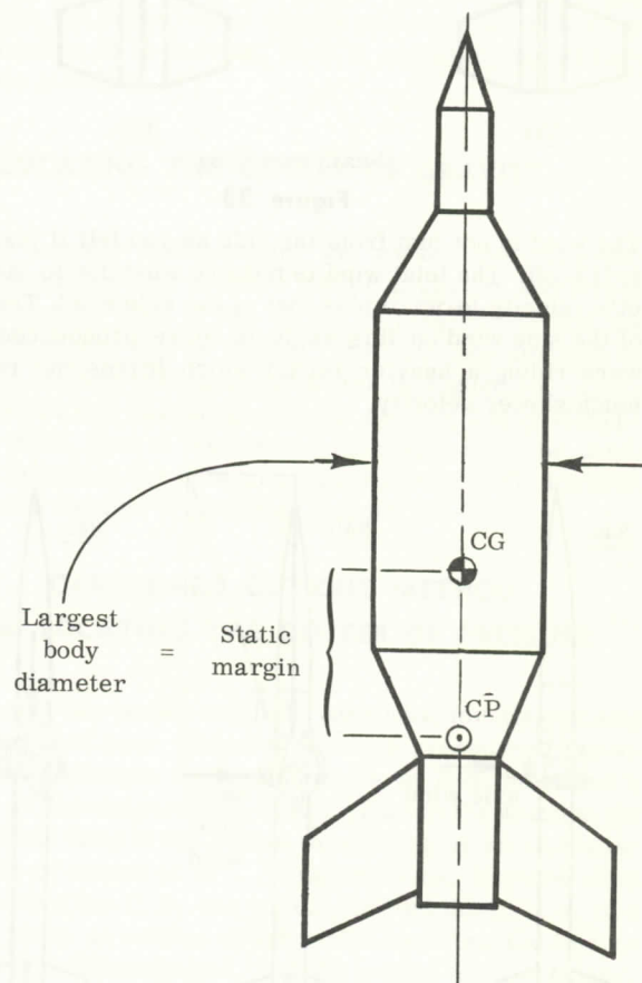
Ideal static margin
