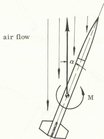
Aerodynamic moment (stable condition)
