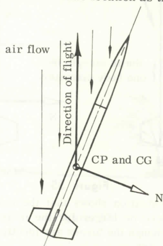
Neutral stability ( M = 0 )
