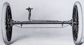
Detail of front axle, showing trussing, steering mechanism and rods; and complete protection afforded the steering gear by the axle itself. Only six moving parts in this steering gear.
