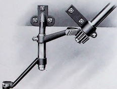
Detail of pinion, affixed to end of steering post, and sector gear. The hexagon nut just above steering-post bracket permits of plenty of adjustment. The long arm of sector casting connects with steering rods. (See cut of front axle on page 30.)
