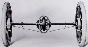
Detail of rear axle showing trussing and oil-tight casing of differential. The large elliptical case is the rear member of the oil-tight engine case.
