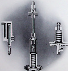
Stanley water indicator, a simple and perfectly reliable device with no moving part.
