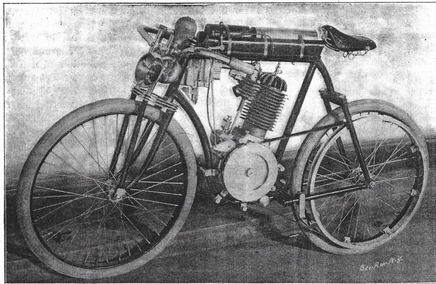
6-Horse Power Marsh Racing Motor Cycle. Mile in 1 M. 2 3-5 S.
