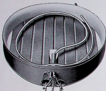
Stanley burner, showing vaporizer and mixing tubes. A drilled cast-iron plate completely encased. In effect a huge burner burner, giving perfect combustion
