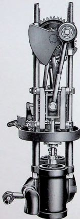
Side view of Stanley engine, showing connecting-rod and bearing, with counterbalance, steam chest cover, and exhaust outlet. The Stanley engine is more completely a roller-bearing engine than any other engine used in an automobile
