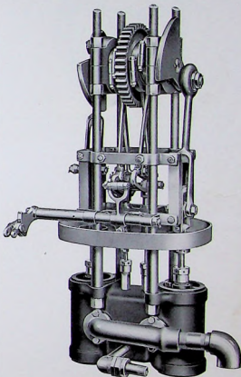
View of Stanley engine, obliquely from above. Showing main bearing, eccentric, link motion, baffle-plate, "hooking-up" device. There are but thirteen moving parts in the Stanley engine
