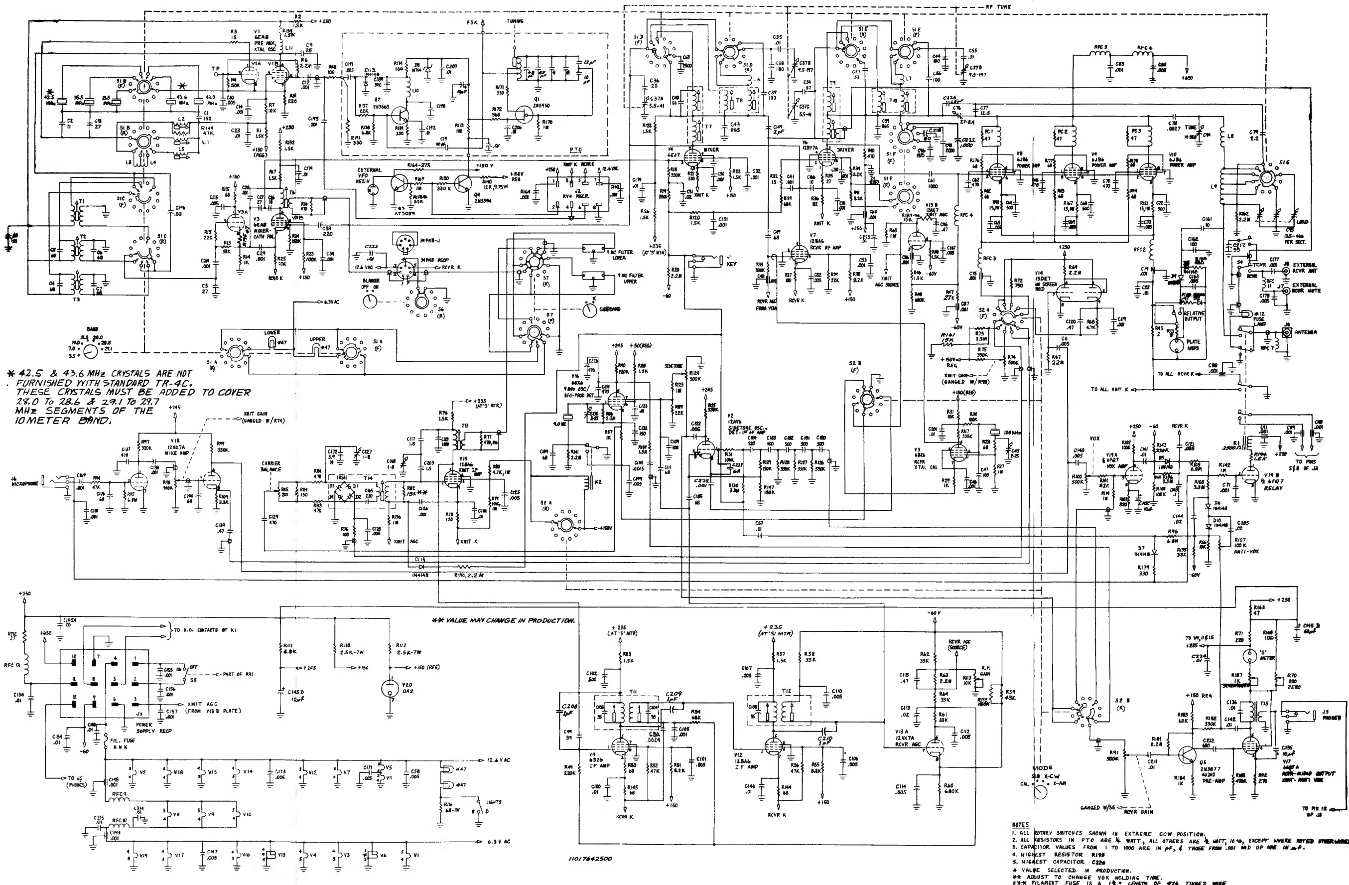
Figure 5–5. TR–4C Schematic
