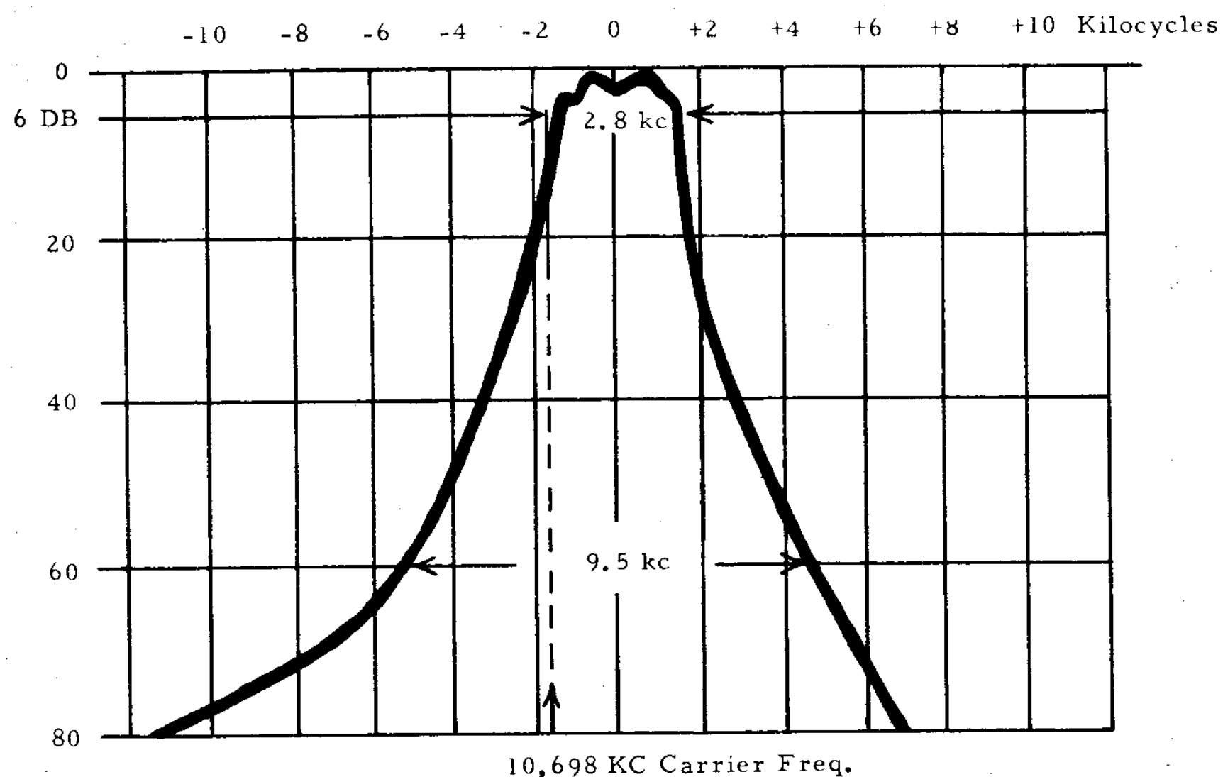
FIGURE 3 CRYSTAL FILTER, TYPICAL CHARACTERISTIC
