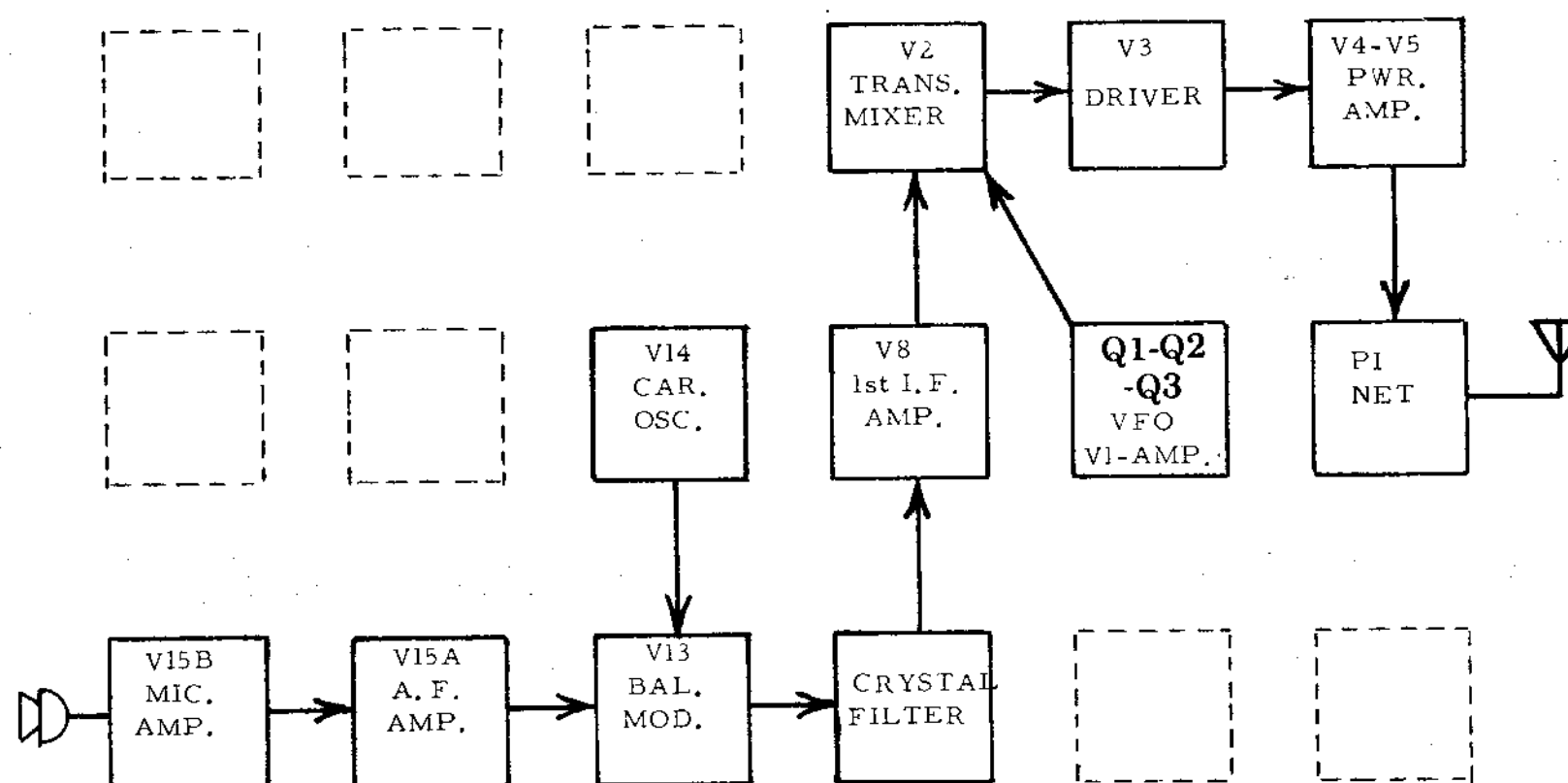
FIGURE 2 BLOCK DIAGRAM, TRANSMIT MODE
