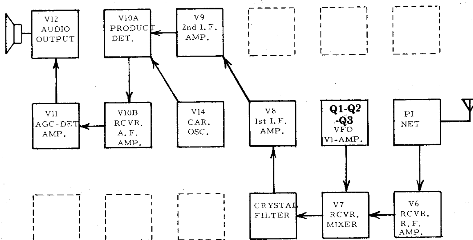
FIGURE 1 BLOCK DIAGRAM, RECEIVE MODE
