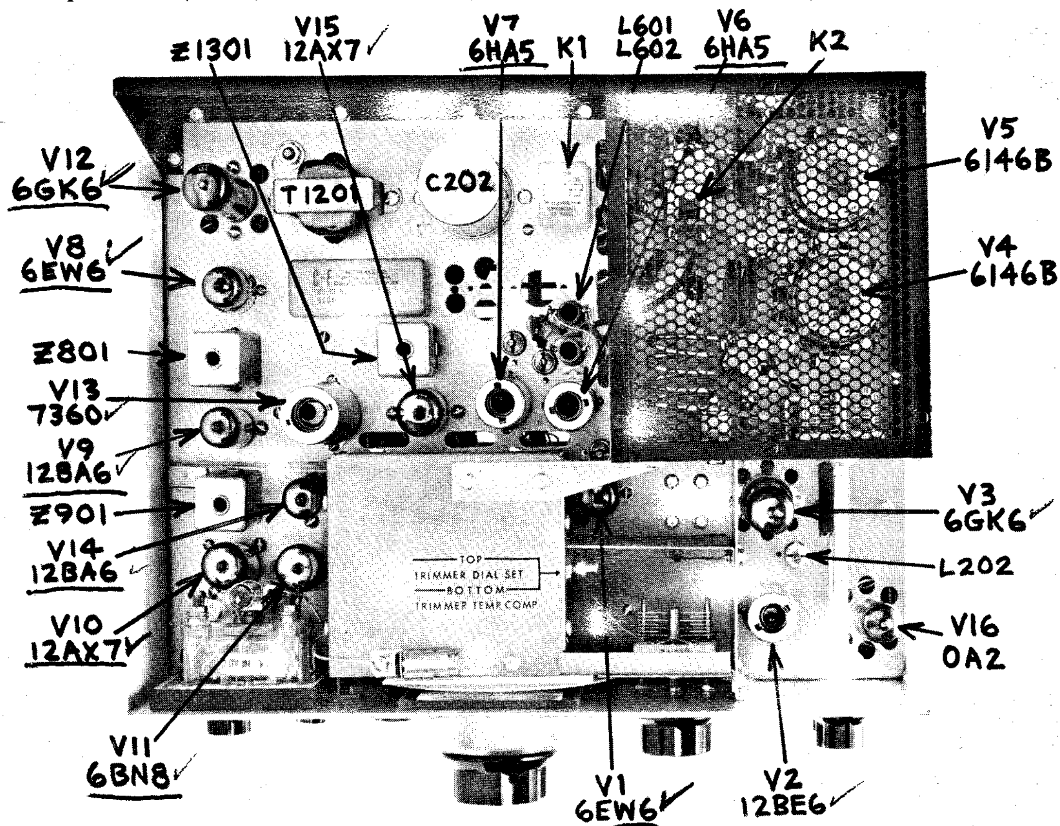
FIGURE 4 TOP VIEW MODEL 250 TRANSCEIVER
