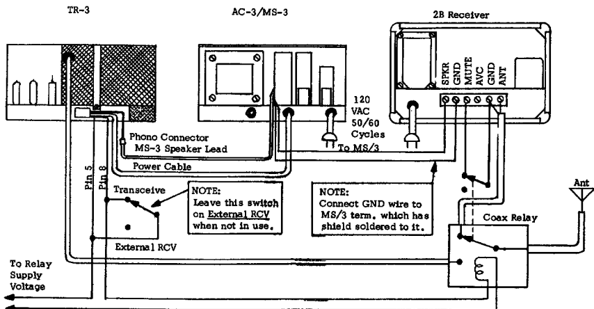
FIG. 3 USING THE TR-3 WITH AN EXTERNAL RECEIVER
