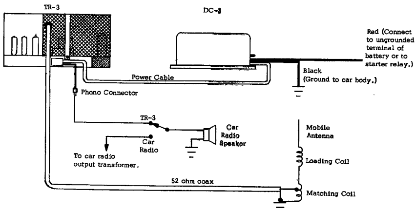
FIG. 4 ELECTRICAL CONNECTIONS FOR MOBILE INSTALLATION OF THE TR-3
