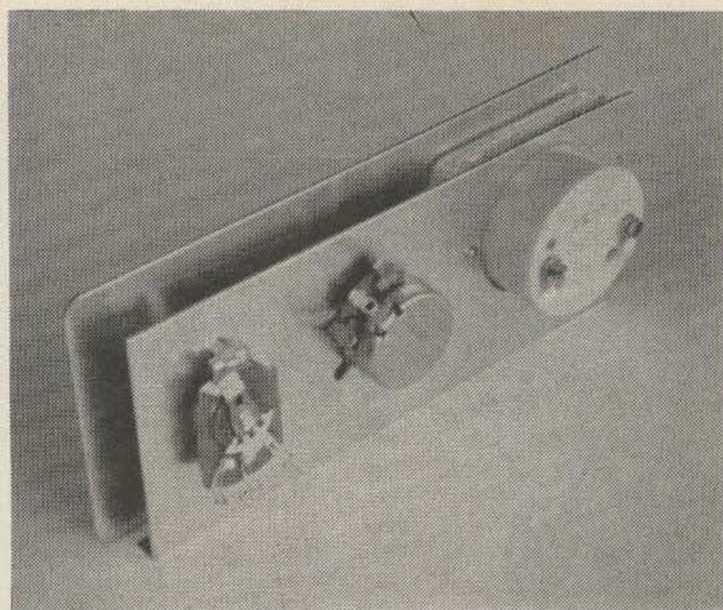
The indicator unit contains a sub-panel to hold the meter, switch and pot, with a "dress" panel for the nomenclature.
