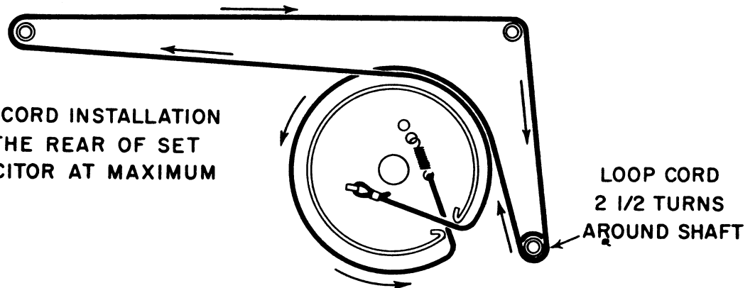
Dial Cord Assembly
