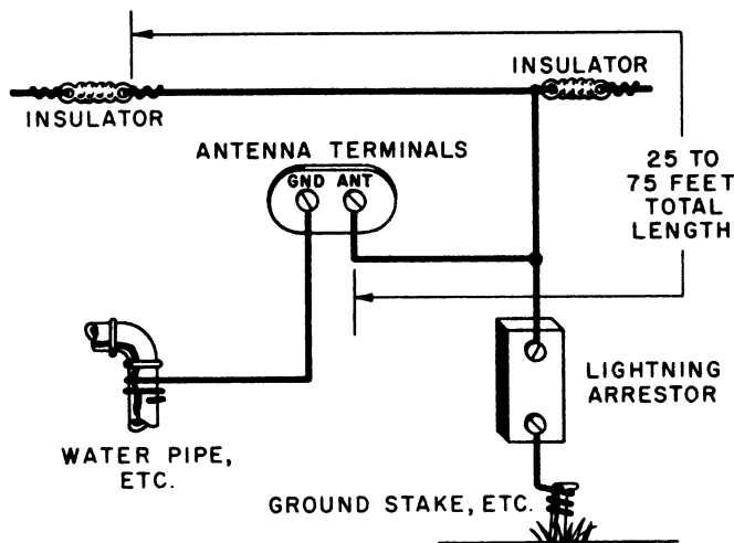
Single Wire Antenna
