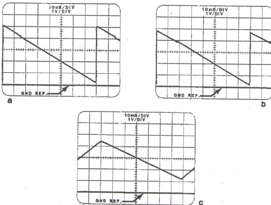
Figure 5-2 Oscilloscope Waveforms
