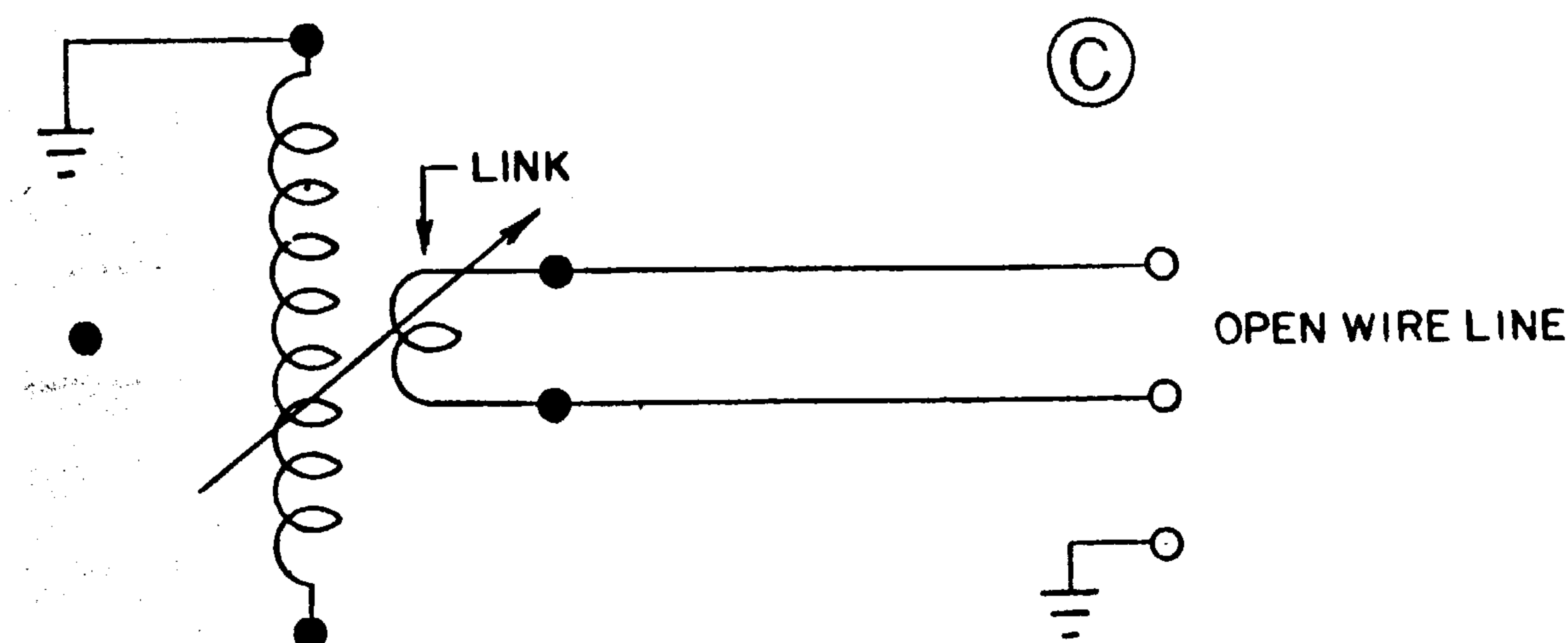
ANTENNA AND FEED LINE CONNECTIONS
