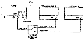
USING THE T-175 WITH A SEPARATE TRANSMITTER/RECEIVER
