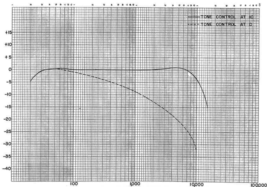
Figure No. 3. Audio Amplifier Frequency Response
