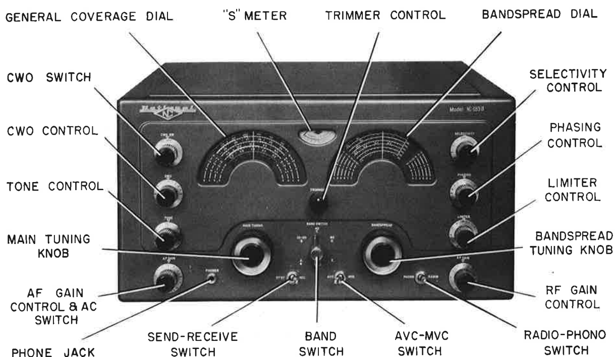
Figure No. 7. Front View of Receiver, Front Panel Control Identification
