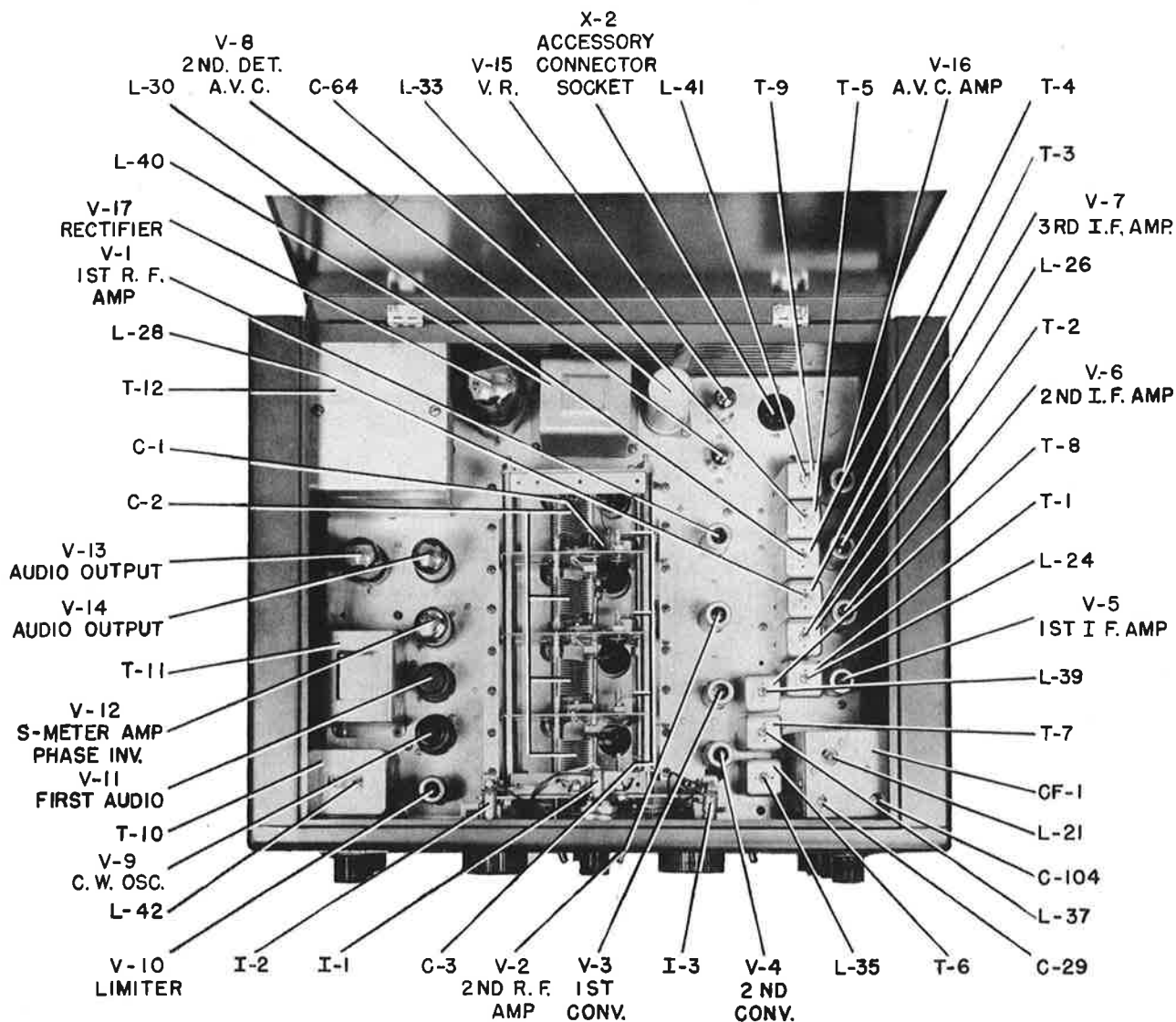
Figure No. 9. Top View of Receiver
