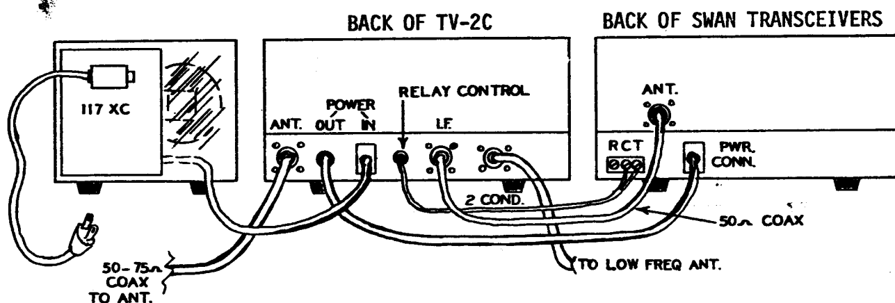
TV-2C CABLE CONNECTIONS, REAR VIEW
