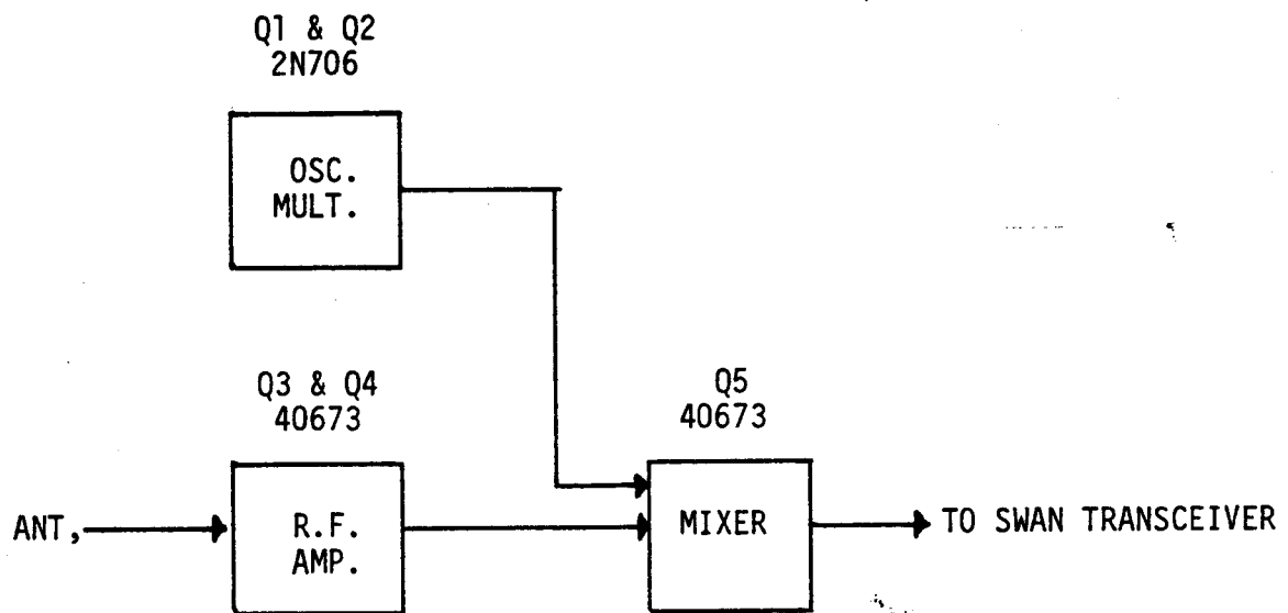
RECEIVE BLOCK DIAGRAM
