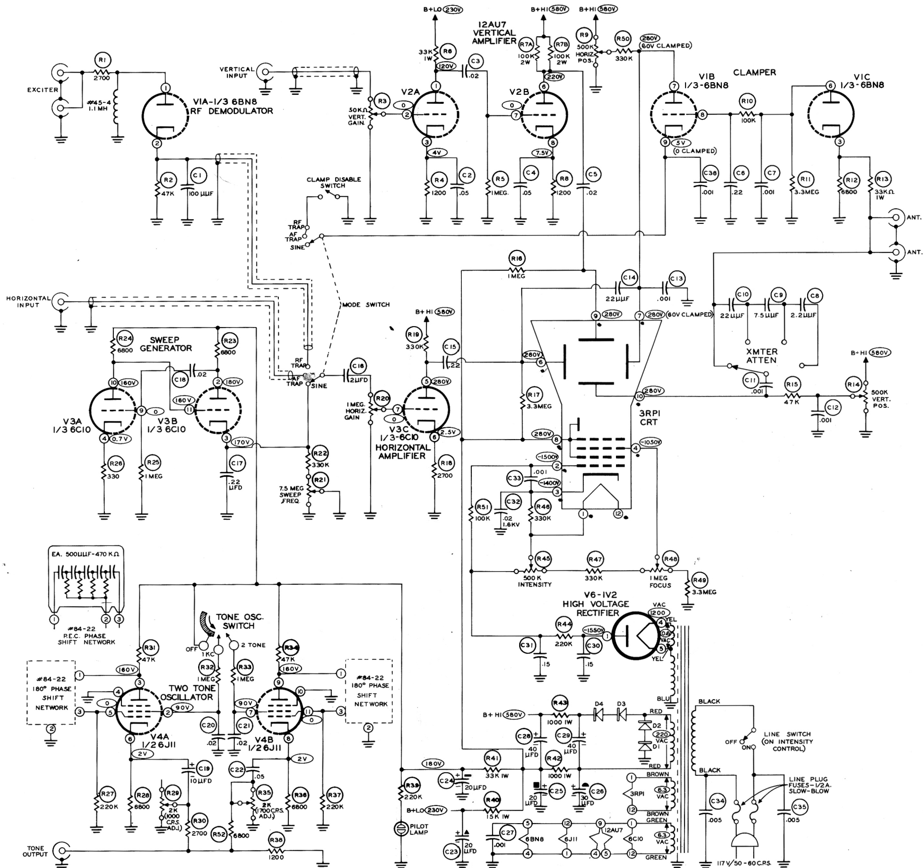
SCHEMATIC OF THE HEATHKIT® MONITOR SCOPE MODEL HO-10
