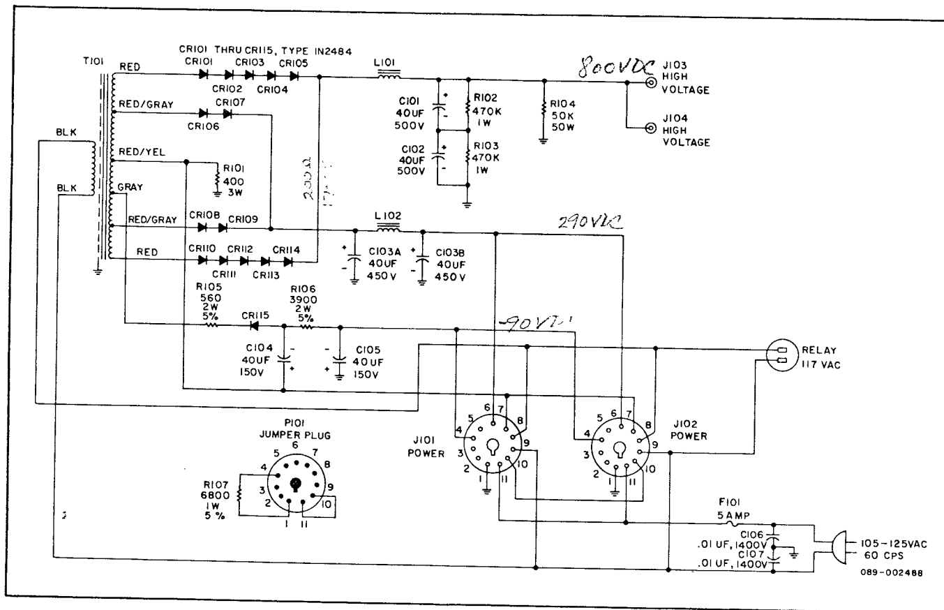
Figure 15. Schematic Diagram of Model P-26 Power Supply.
