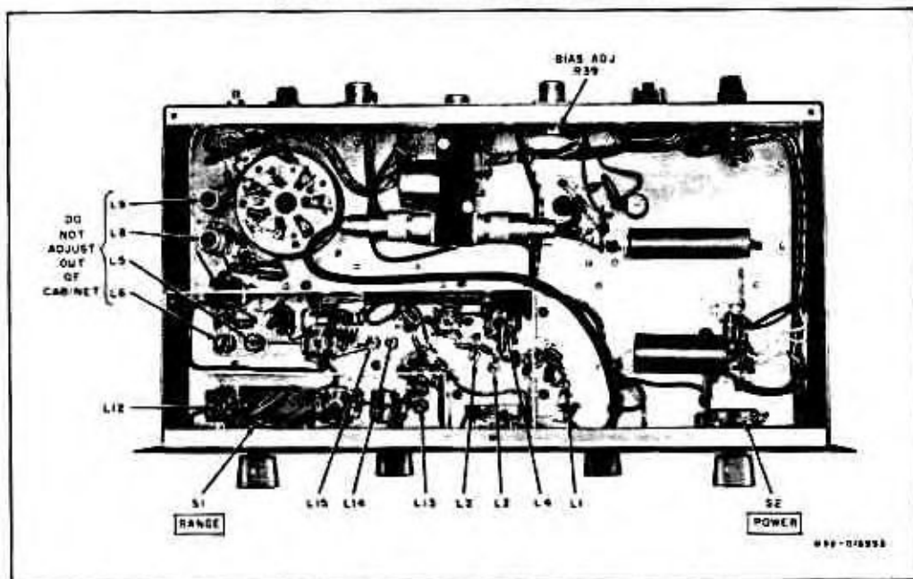
Figure 10. Bottom View of Transverter Chassis.
