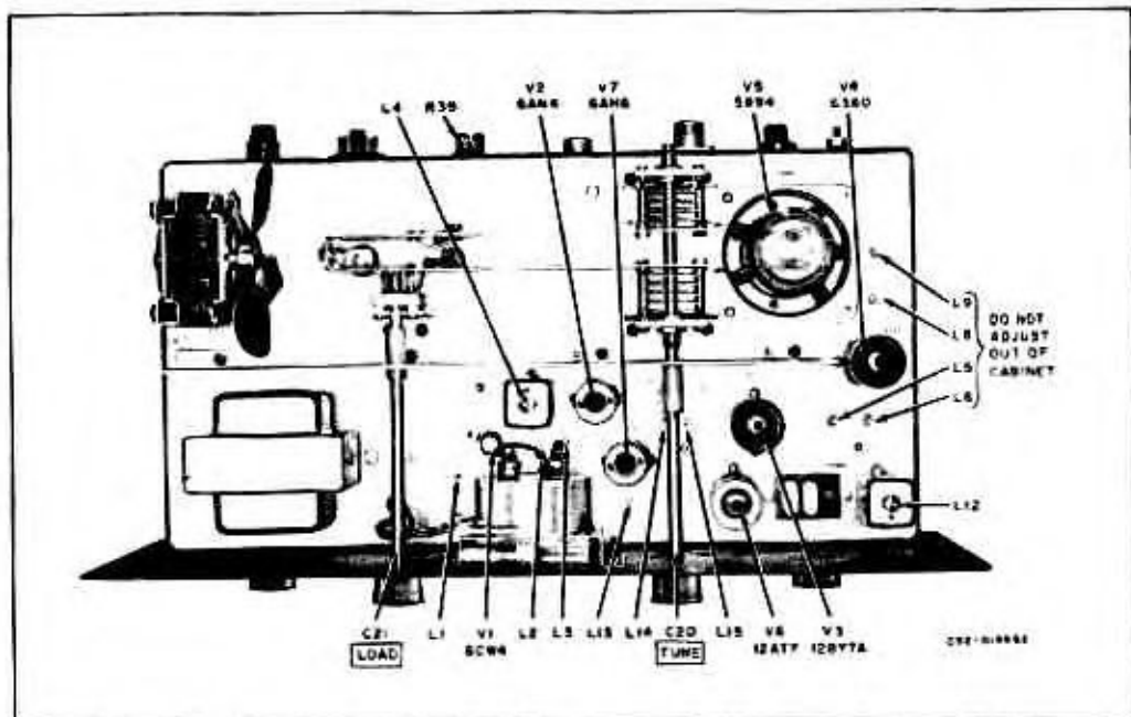
Figure 9. Top View of Transverter Chassis.
