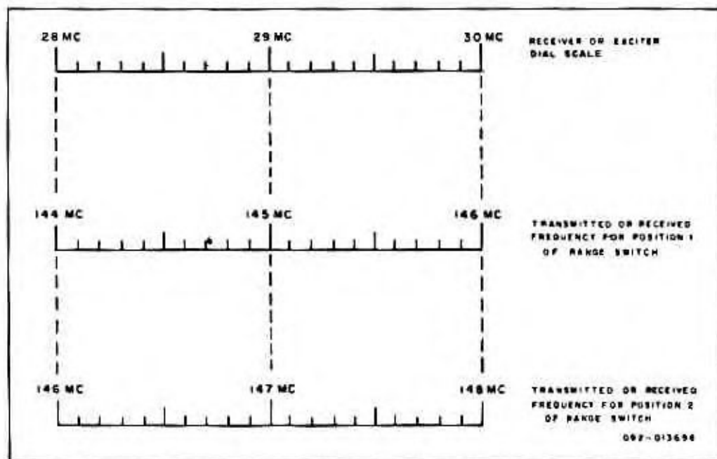
Figure 5. Frequency Conversion (Dial Scale Interpolation).
