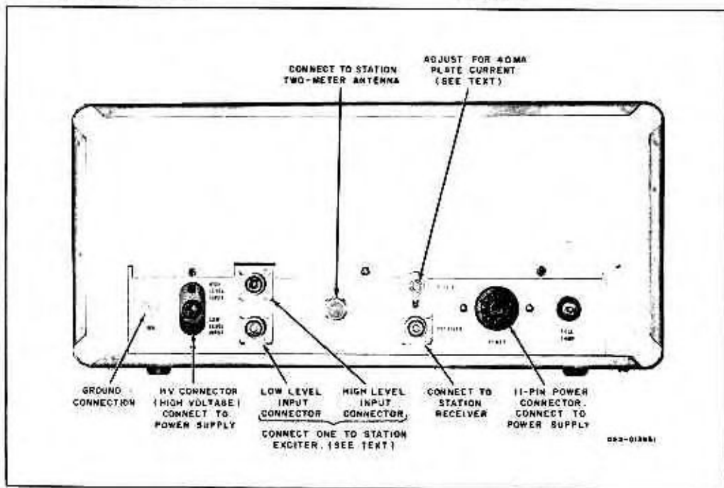
Figure 2. Rear View of Transverter, Showing Connectors.
