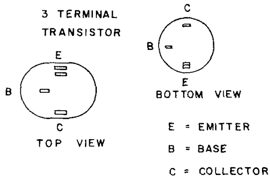
3-TERMINAL TRANSISTOR SOCKET (BOTTOM VIEW)
