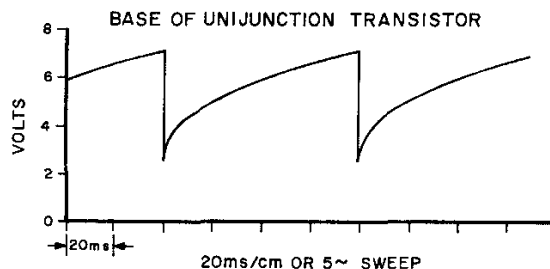
SWEEP WAVEFORM AT BASE OF UNIUNCTION TRANSISTOR
