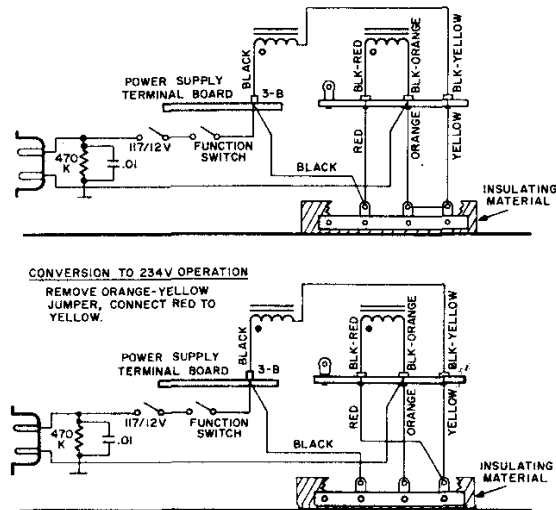
117/234-VOLT AC OPERATION, WIRING DIAGRAMS
