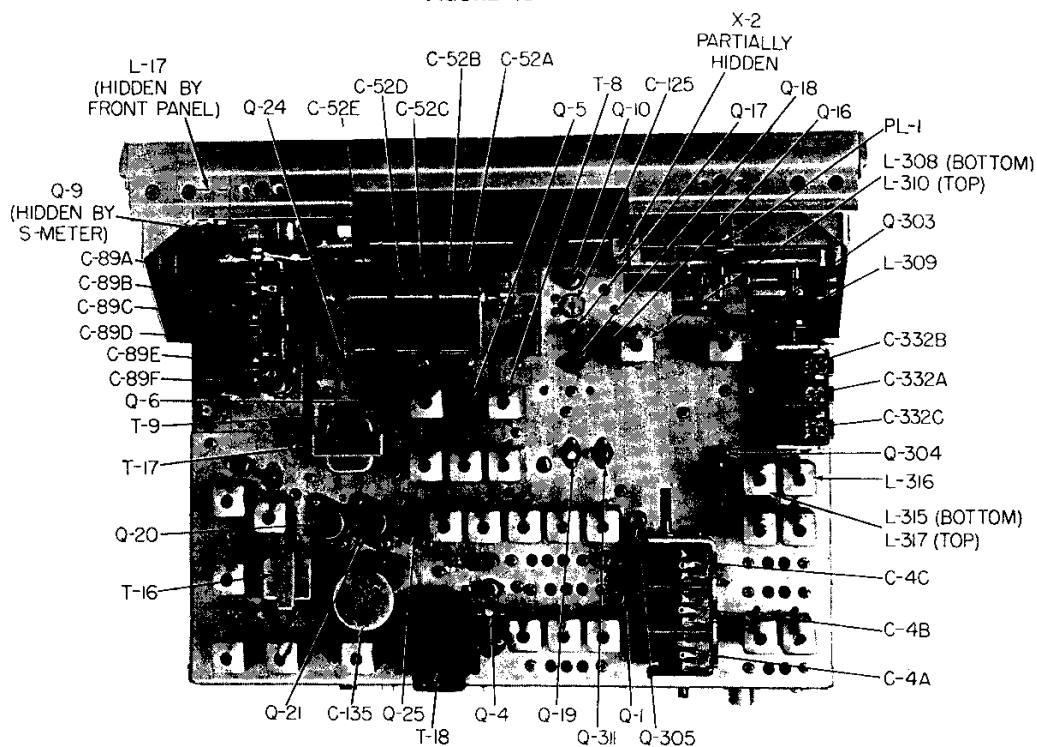
HRO-500 RECEIVER CHASSIS, WITH SYNTHESIZER AND COVERS REMOVED, TOP VIEW
