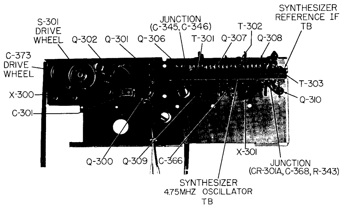
SYNTHESIZER CHASSIS, FRONT VIEW
