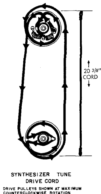
DRIVE CORD—SYNTHESIZER TUNE FIGURE 43
