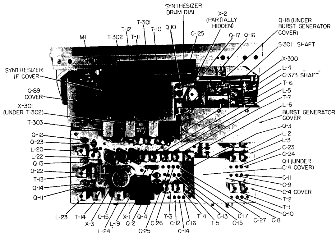
HRO-500 RECEIVER CHASSIS, TOP VIEW
