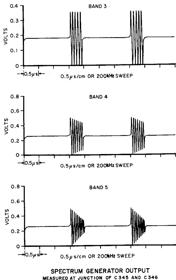
SPECTRUM GENERATOR, OUTPUT WAVEFORM FIGURE 24
