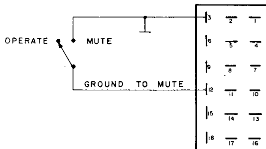
GROUND-REFERENCE MUTING
