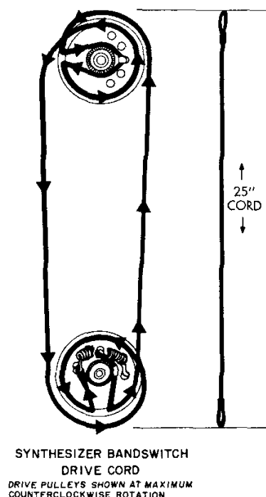
DRIVE CORD—SYNTHESIZER BANDSWITCH FIGURE 44
