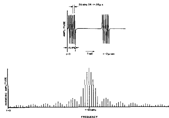
SPECTRUM GENERATOR, FREQUENCY AND TIME DOMAIN
