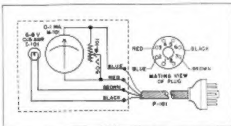
Figure No. 7. Schematic Diagram--SM-57 Tuning Meter
