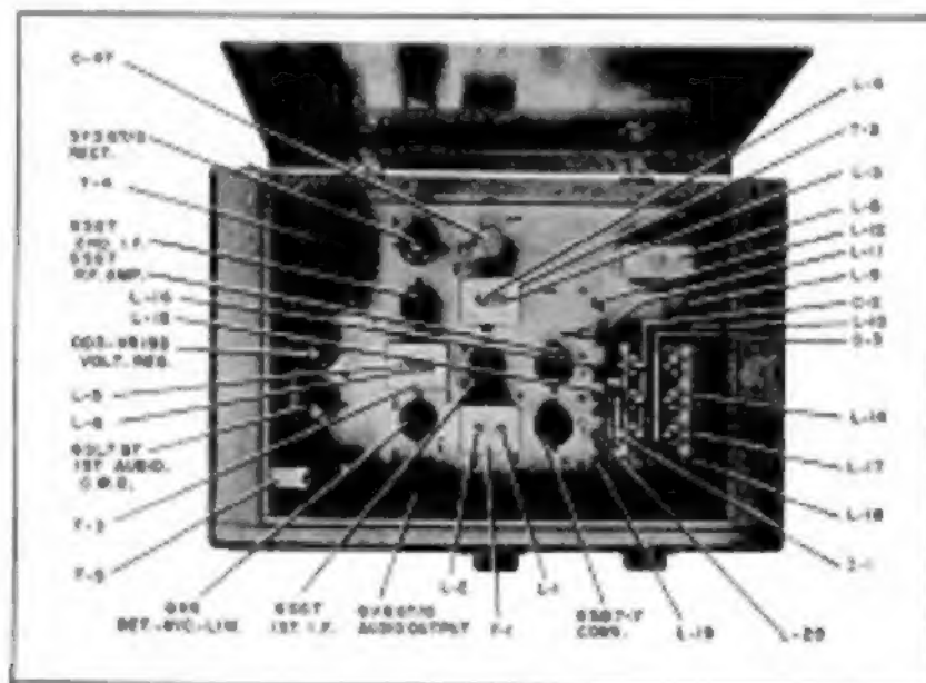
Figure No. 2. Top View of Receiver
