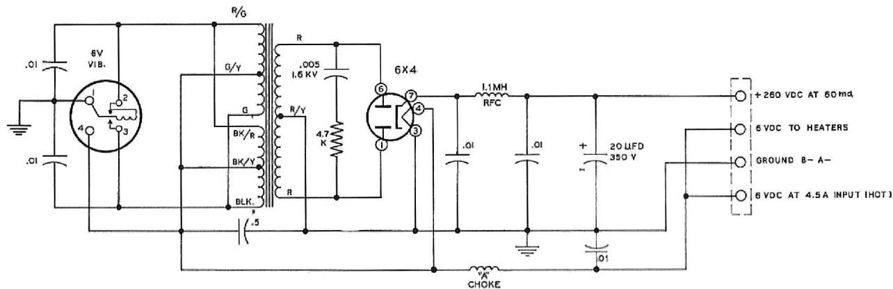
HEATHKIT 6 VOLT VIBRATOR POWER SUPPLY MODEL VP-1-6
