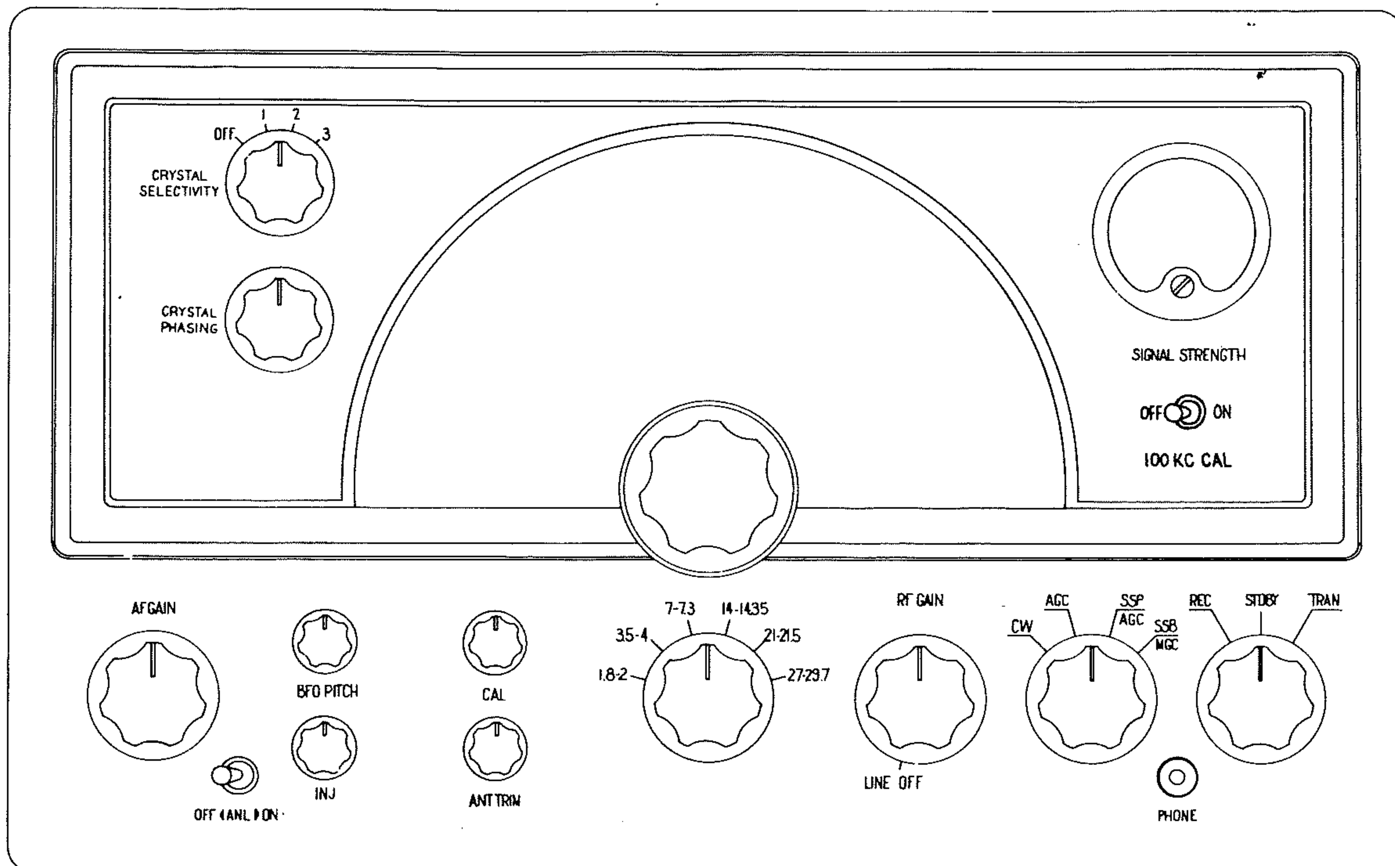
Fig. 2 — Front Panel Layout
