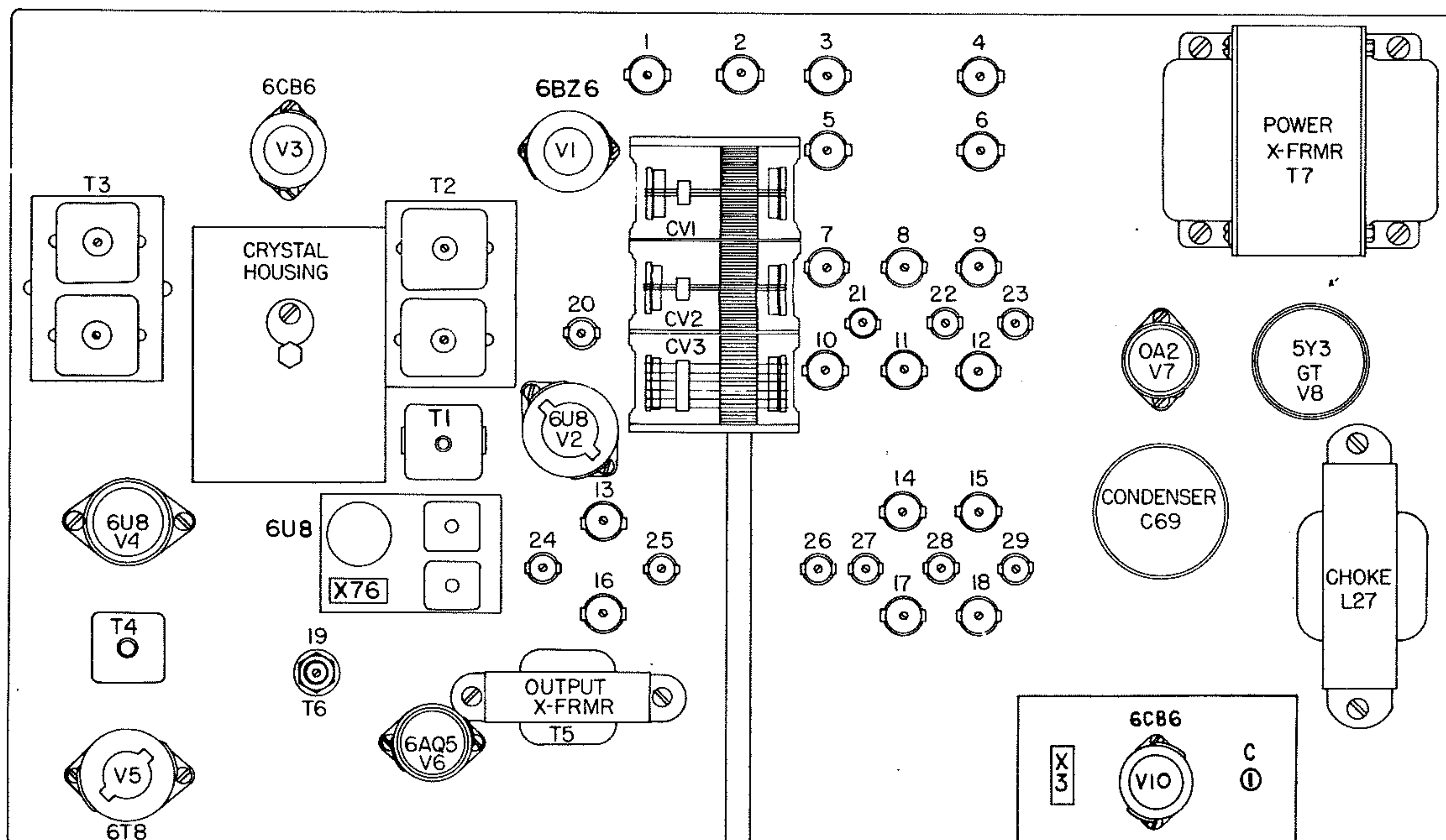
TRIMMER & COIL ADJUSTMENT LOCATIONS
