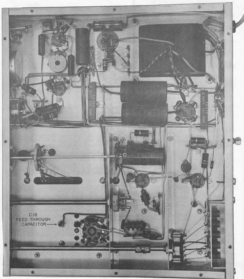
PICTORIAL 12 COMPLETED WIRING — UNDERCHASSIS VIEW
