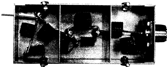
COMPLETED WIRING
