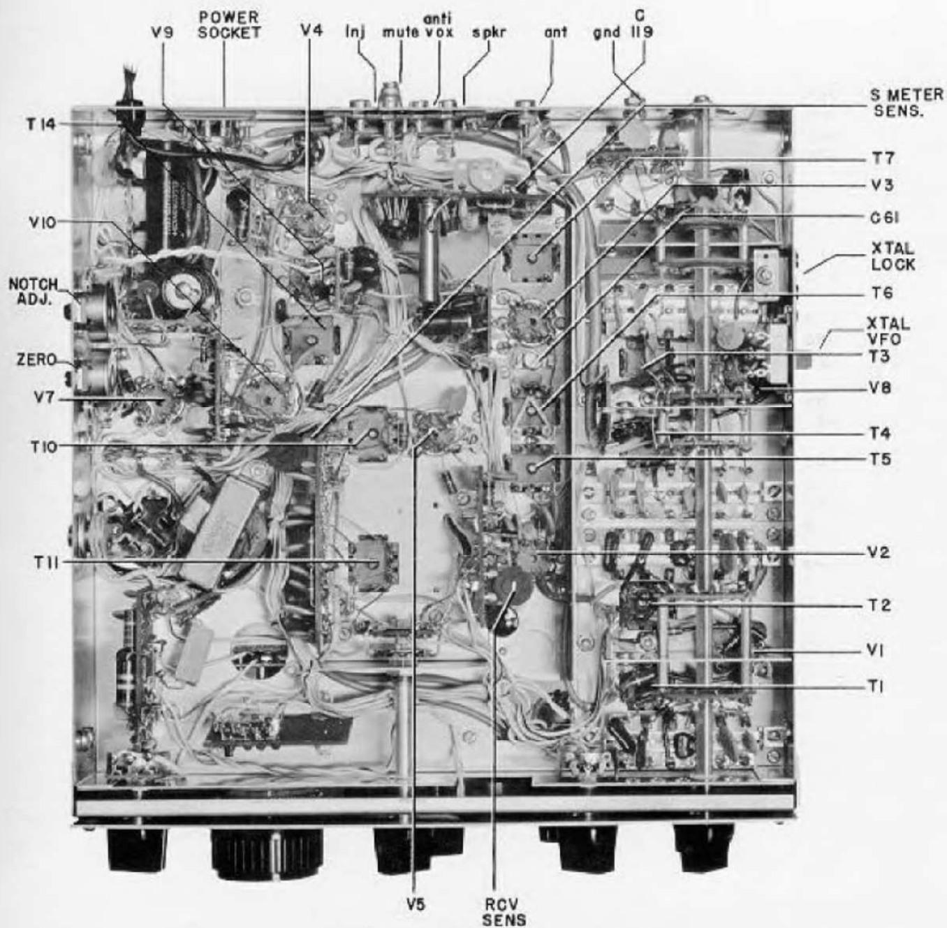
FIGURE #13 BOTTOM VIEW
