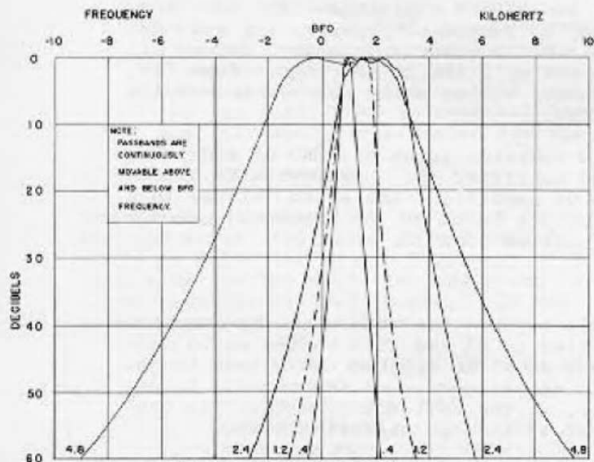
FIGURE #7 — SELECTIVITY CURVES
