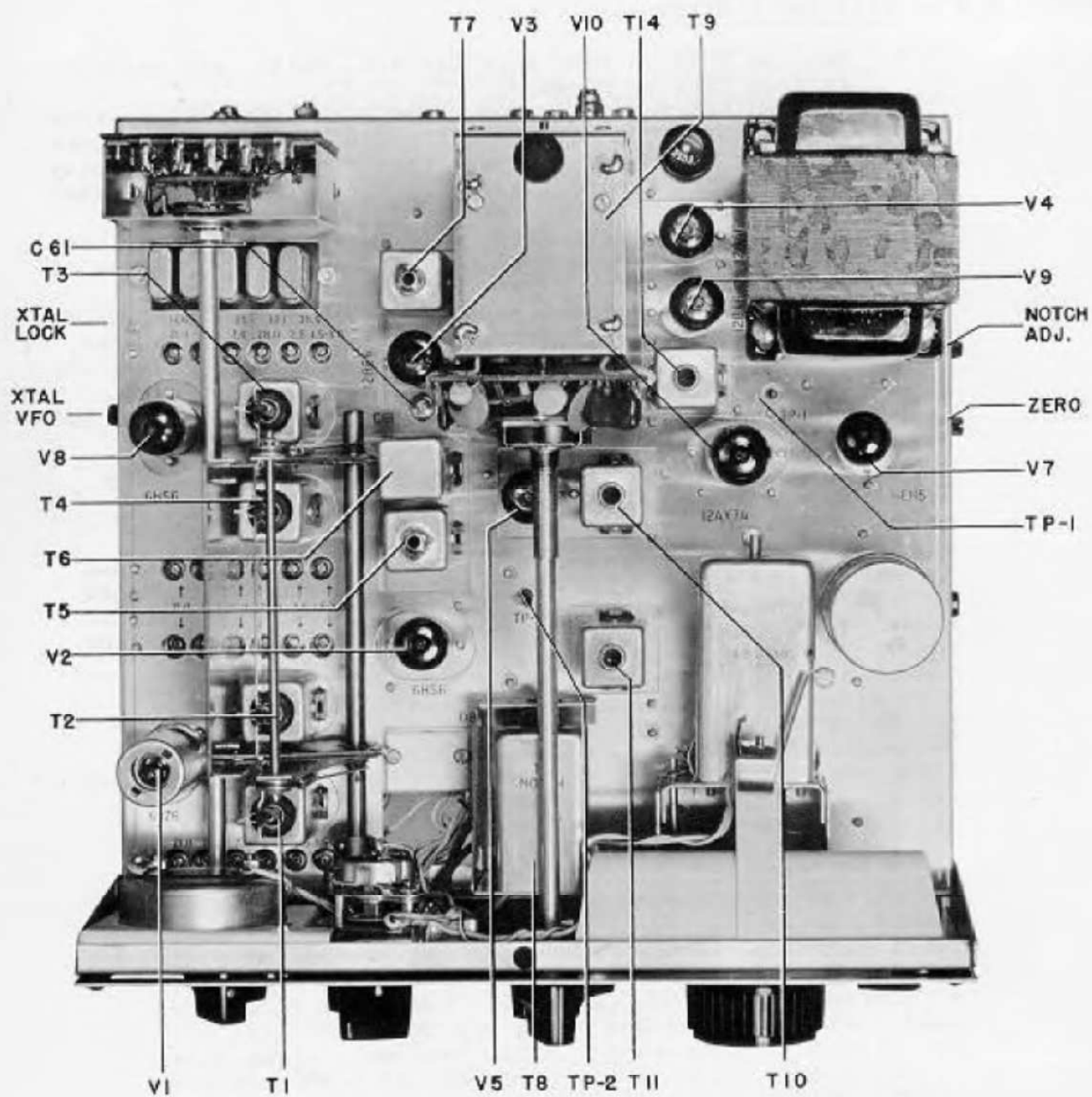
FIGURE #12 TOP VIEW
