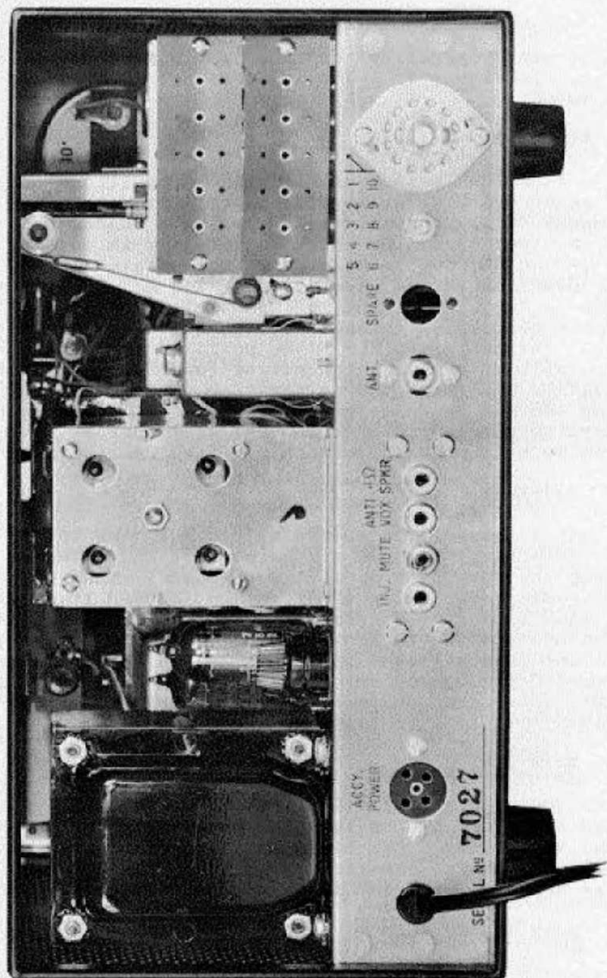
FIGURE #4 REAR VIEW
