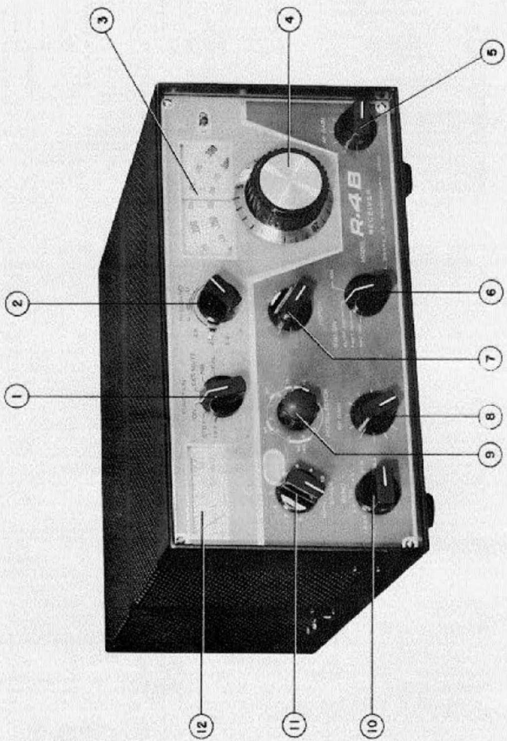
FIGURE #3 FRONT PANEL
