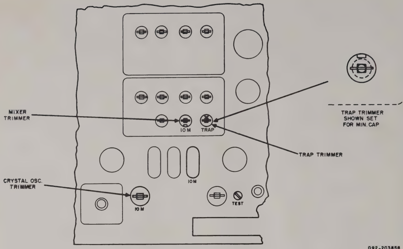
Figure 6. 10 Meter Band Adjustments
