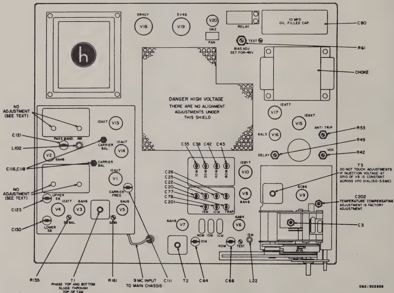
Figure 9. Top Chassis Alignment Points
