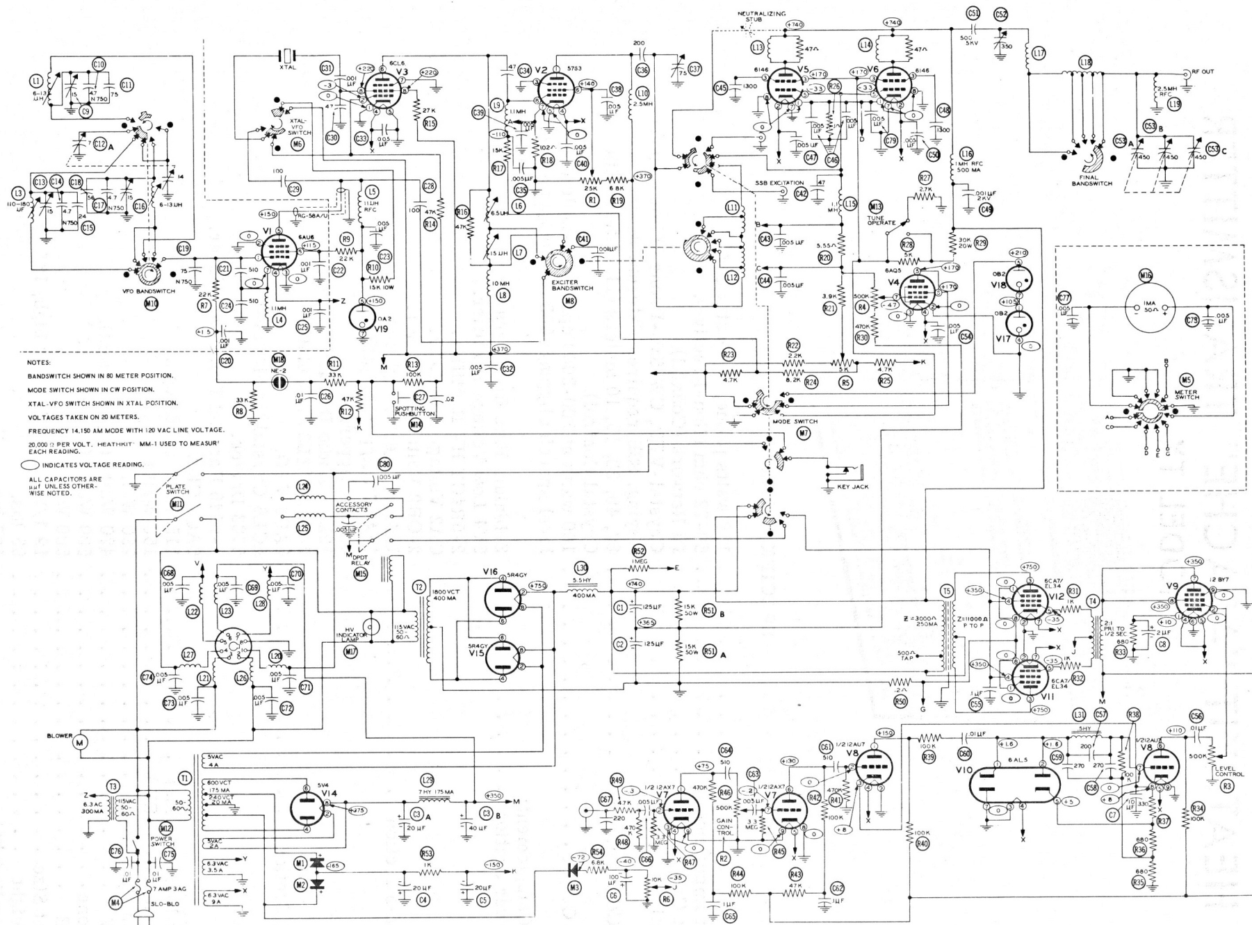
HEATHKIT "APACHE" TRANSMITTER MODEL TX-1
