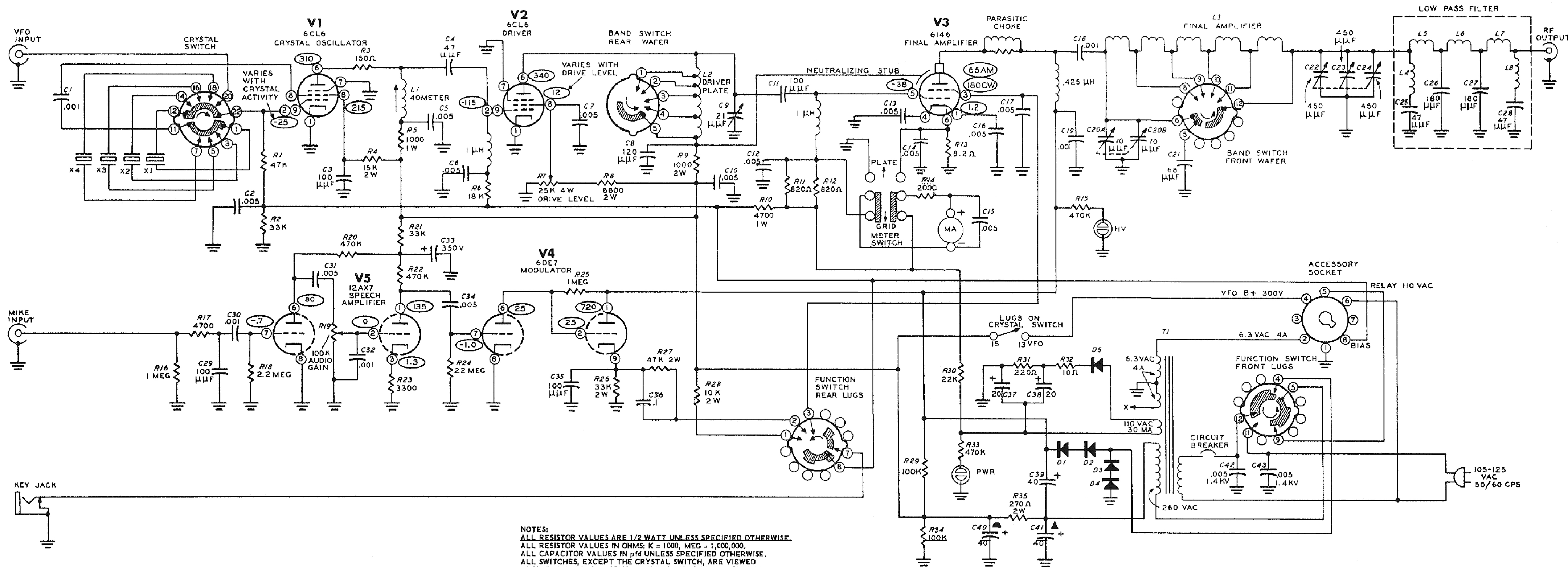
Schematic of the HEATHKIT® AMATEUR TRANSMITTER Model DX-60A
