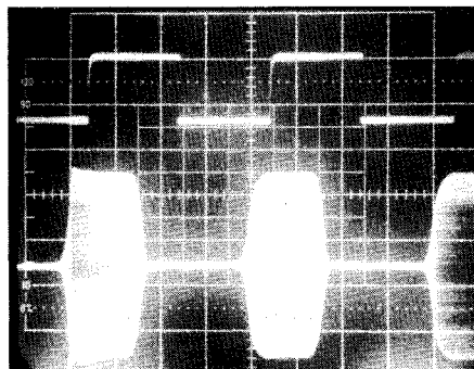
Fig 3—CW-keying waveforms for the TS-850S in the semi-break-in mode (A) and the full-break-in mode (B). The upper traces are the actual key closures; the lower traces are the RF envelopes. Horizontal divisions are 20 ms. The transmitter was being operated at 100 W output on 14.02 MHz. Other than a somewhat hard first keyed element (in both VOX and full-break-in modes), the TS-850S's CW keying shaping is excellent.
