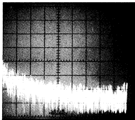
Fig 4—Spectral display of the TS-850S transmitter output during composite-noise testing. Power output is 100 W at 3.52 MHz (A) and 100 W at 14.02 MHz (B). Vertical divisions are 10 dB; horizontal divisions are 2 kHz. The scale on the spectrum analyzer on which these photos were taken is calibrated so that the log reference level (the top horizontal line on the scale) represents -60 dBc/Hz and the baseline is -140 dBc/Hz. Composite-noise levels between -60 and -140 dBc/Hz may be read directly from the photographs. The carrier, off the left edge of the photographs, is not shown. These photographs show composite transmitted noise at frequencies 2 to 20 kHz offset from the carrier.
