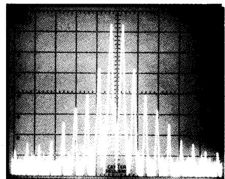
Fig 2—Worst-case spectral display of the TS-850S transmitter during two-tone intermodulation distortion (IMD) testing. Third-order products are approximately 28 dB below PEP output, and fifth-order products are approximately 40 dB down. Vertical divisions are 10 dB; horizontal divisions are 2 kHz. The transceiver was being operated at rated output (100 W PEP) at 14.25 MHz.
