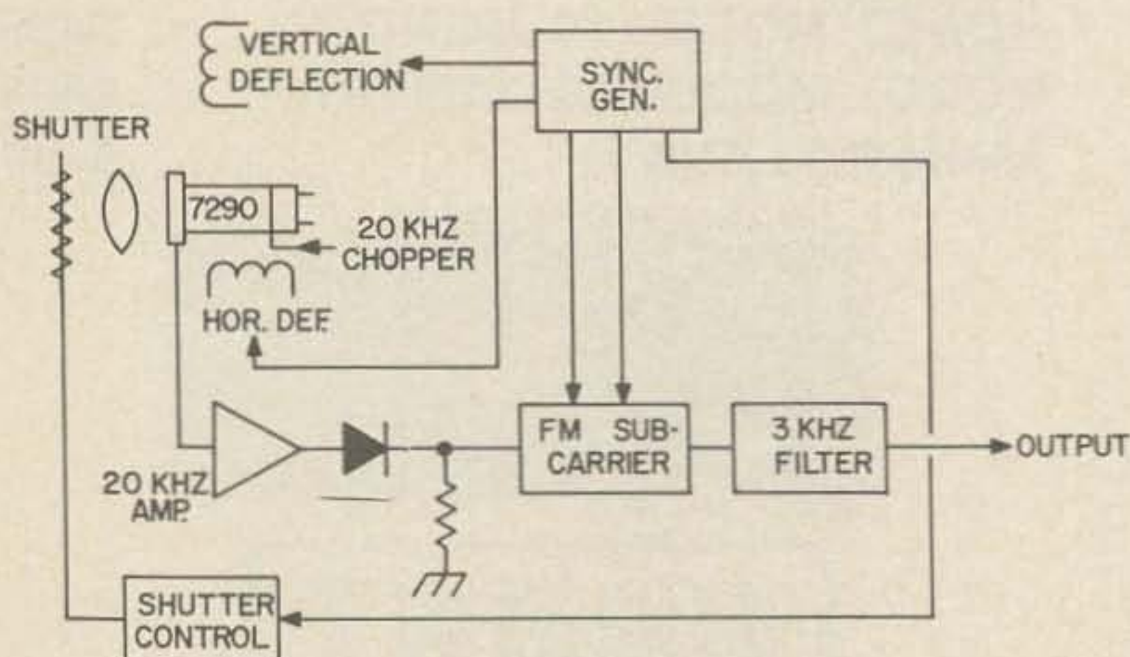
Fig. 1-10. 7290 shuttered camera.
