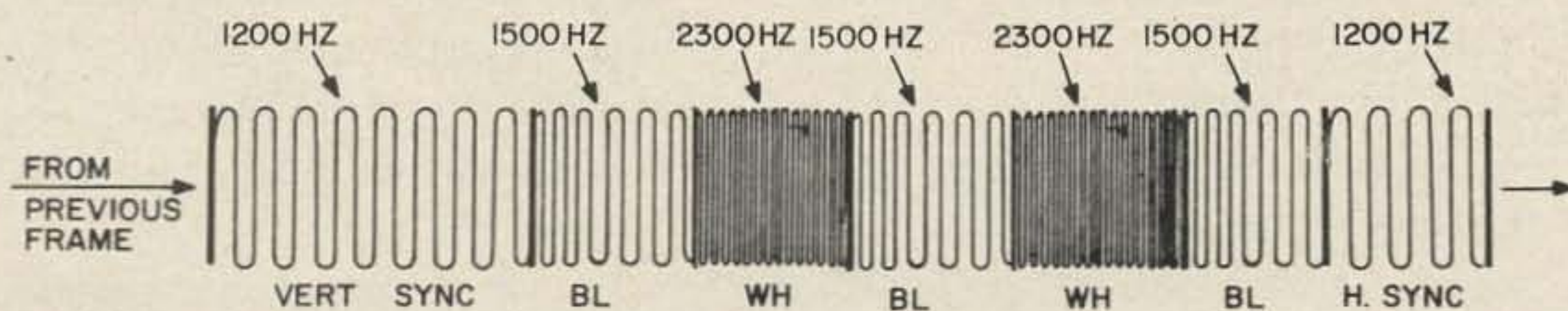
Fig. 1-6. Composite FM subcarrier modulated with composite sync and video. The composite video signal consists of a midrange audio tone ranging from 1200 to 2300 Hz and is processed in the transmitter and receiver just like a voice
