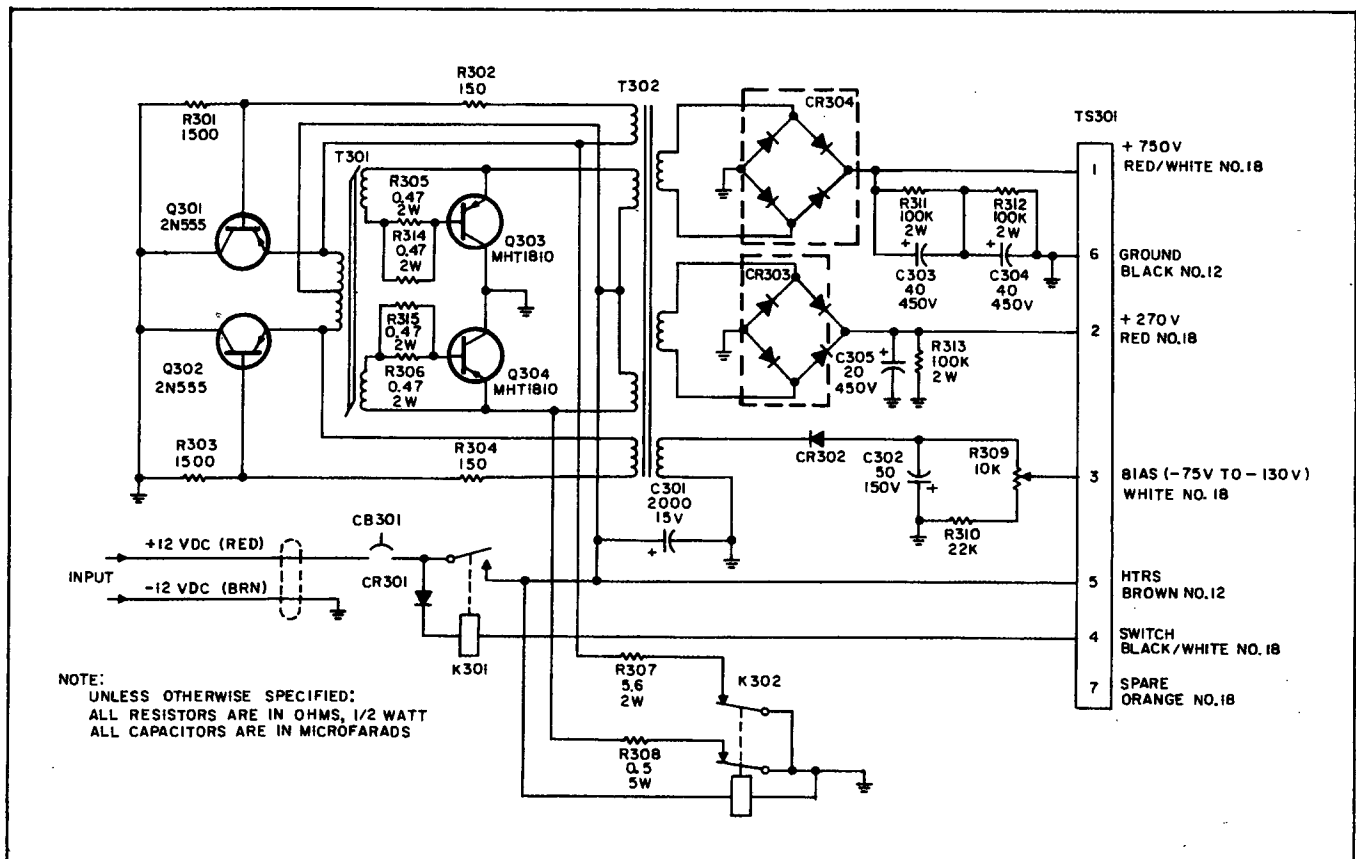
Figure 19. Schematic Diagram of Model PS-500-DC Power Supply.
