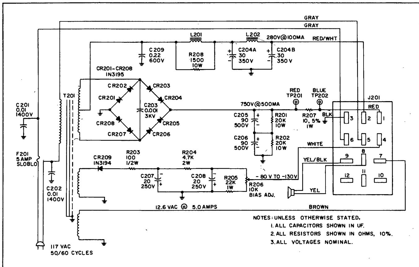
Figure 16. Schematic Diagram of Model PS-500-AC Power Supply.
