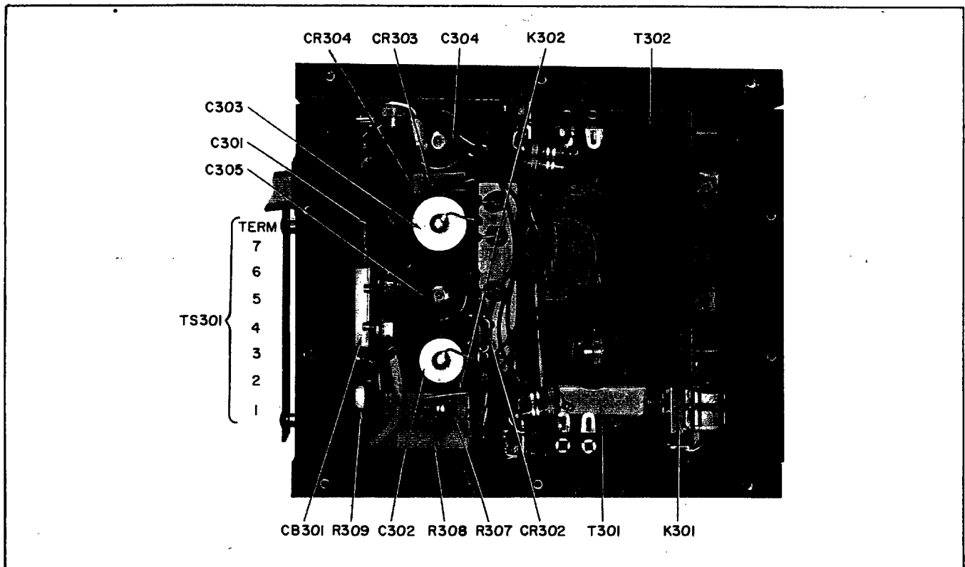
Figure 18. Internal View of Model PS-500-DC Power Supply.
