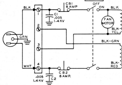
SCHEMATIC OF THE HEATHKIT® LINEAR AMPLIFIER MODEL SB-200
