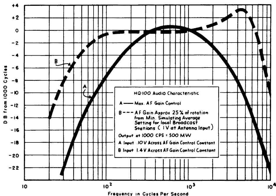
Figure 6. Auto-Response Curve
