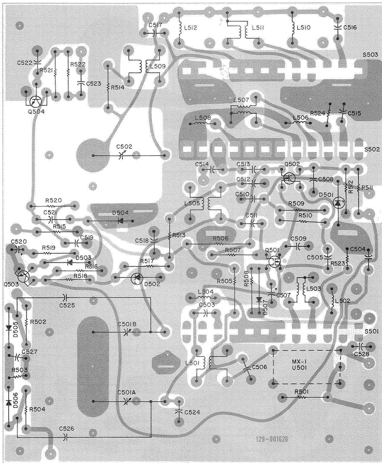
Figure 7-8. Component Layout, Pre-Selector/ALC Module.
