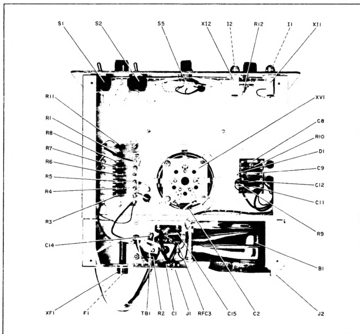
Figure 4. Bottom View of Linear Amplifier, Showing Component Locations.
