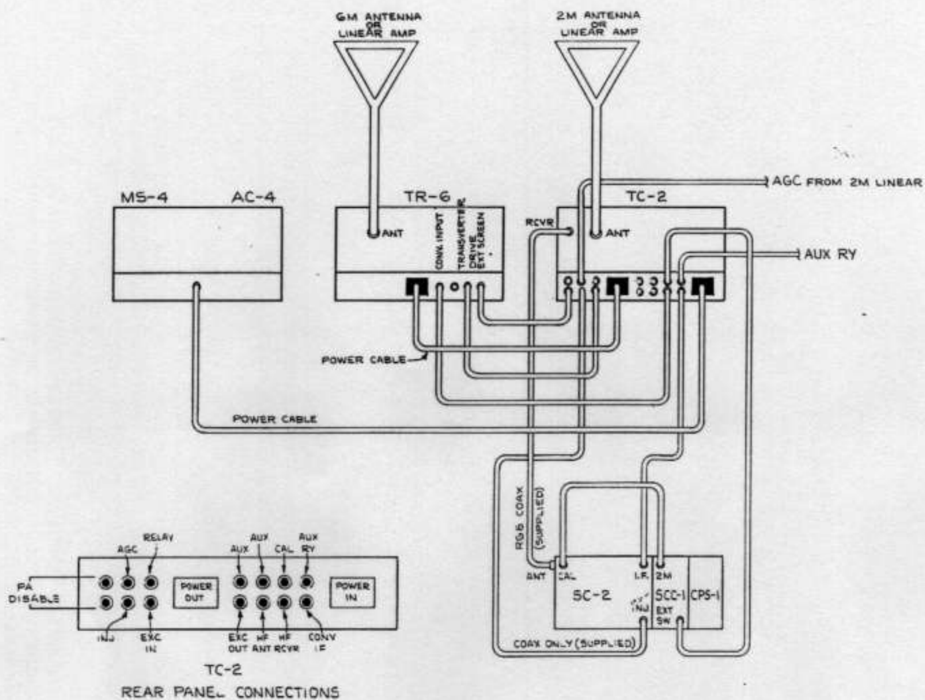
FIGURE 9 INTERCONNECTION WITH TR-6 AND SC-2
