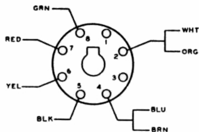
CABLE CONNECTOR
