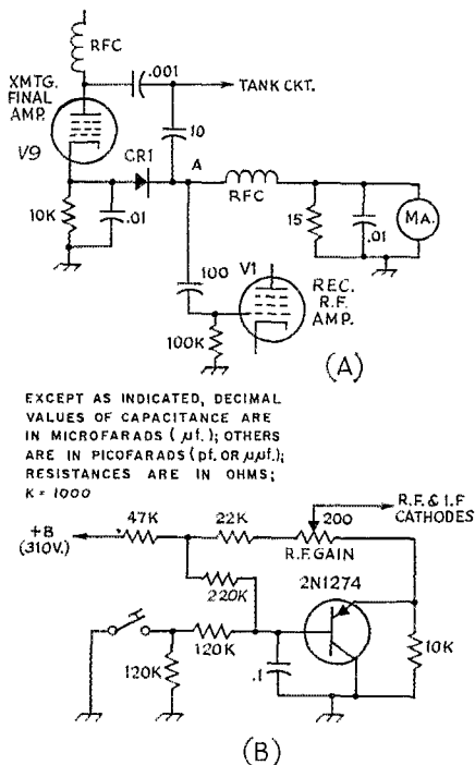
Fig. 2—A—Automatic transmit-receive switching circuit. CR1 shorts the receiver input to ground when the transmitting final amplifier is operating, but becomes nonconducting while receiving. B—Muting circuit, using a transistor to switch extra cathode bias (voltage drop in the 10K resistor) into two receiver stages when the key is pressed. Point C is connected to the negative keying bias (about 100 volts) and the tone oscillator.
