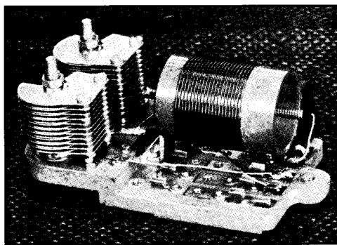
A MEDIUM-FREQUENCY R.F. COIL UNIT REMOVED FROM ITS SHIELD
