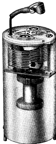
The improved model National Air Dielectric condenser-tuned I.F. transformer, as used in the National FB7A, AG5X and HRO receivers
