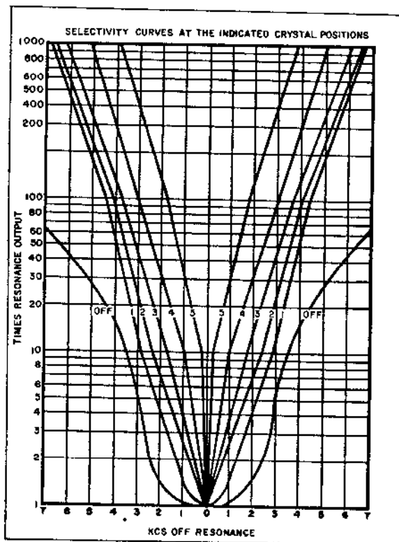
Figure 6. Selectivity Curves
