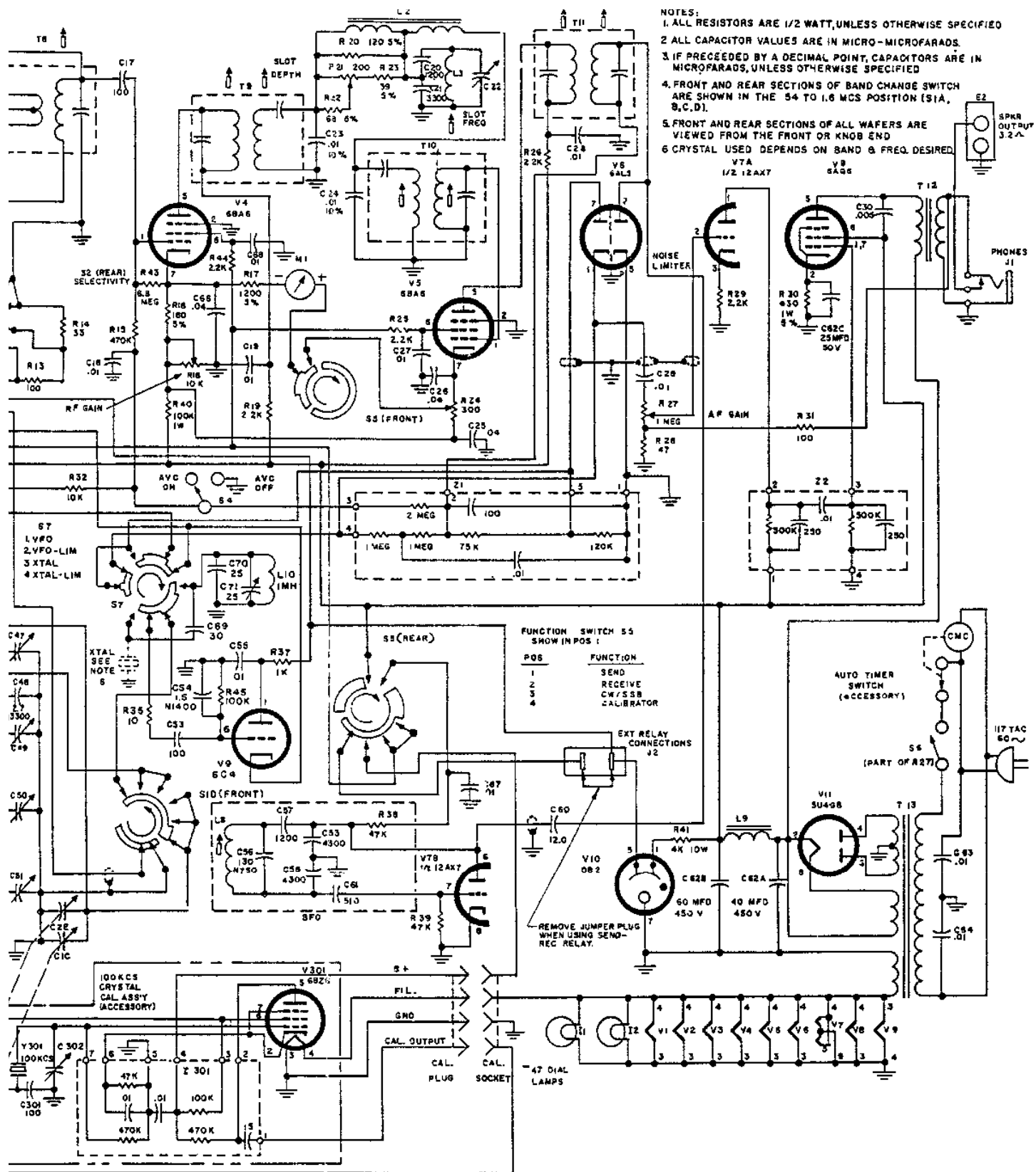
Figure 12. Hammarlund HQ-145X Communications Receiver, Schematic Diagram
