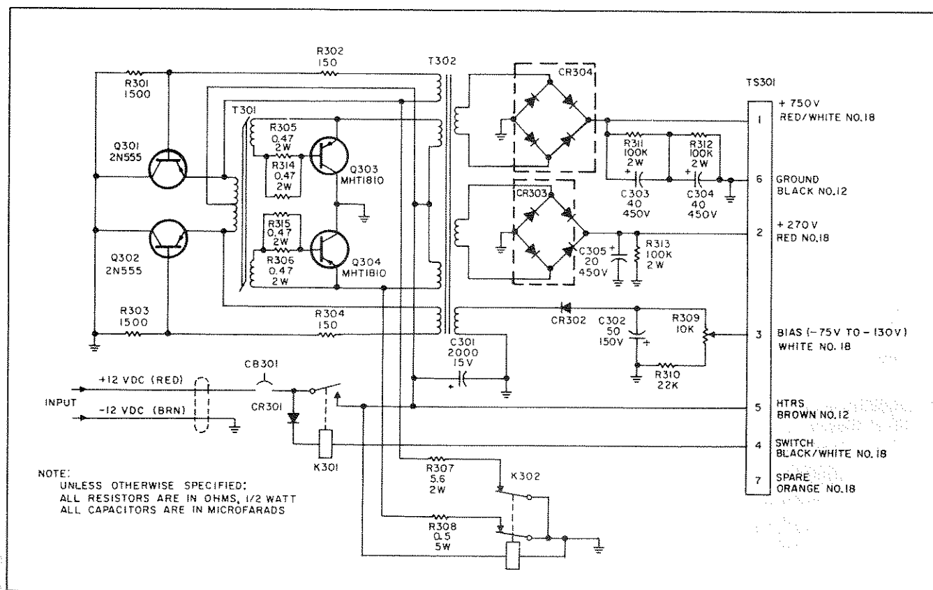
Figure 23. Model PS-500-DC Power Supply, Schematic Diagram.
