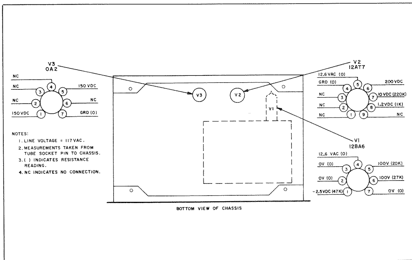
Figure 27. Model HA-20 Voltage and Resistance Chart.
