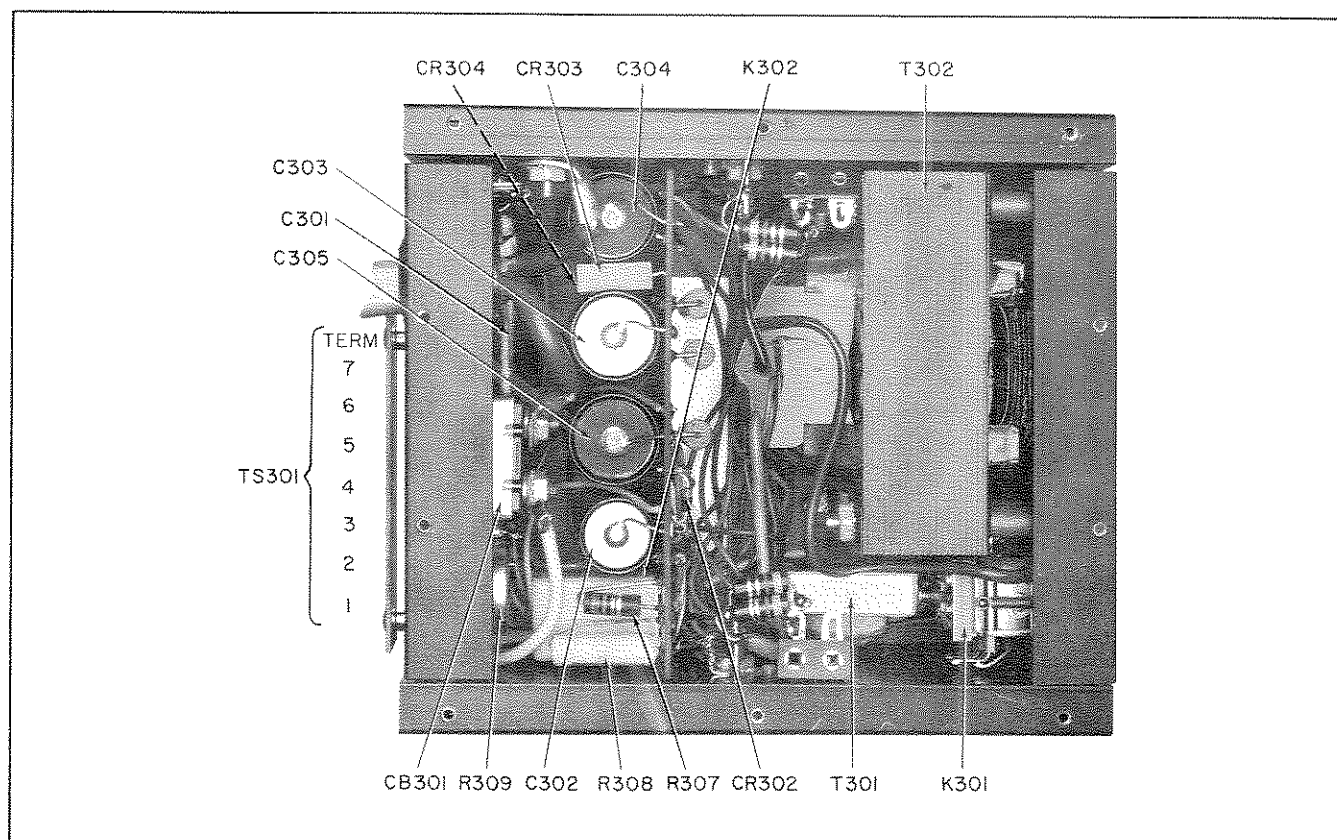
Figure 22. Model PS-500-DC Power Supply, Bottom View.
