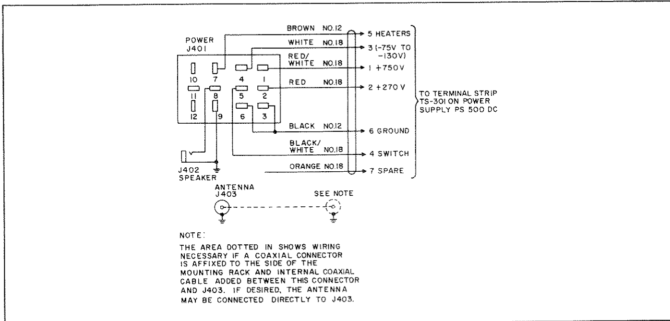
Figure 25. Model MR-400 Mobile Rack, Schematic Diagram.
