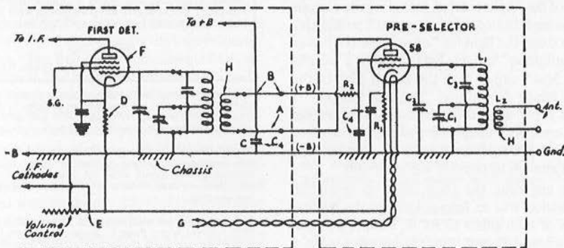
CIRCUIT OF THE ONE-STAGE PRE-SELECTOR AMPLIFIER
