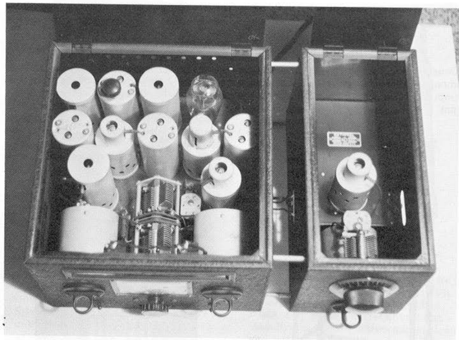
Top view of FB7X. The pre-selector is at right.
