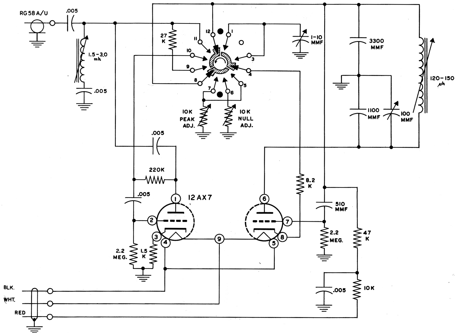
SCHEMATIC OF Q MULTIPLIER QF-1
