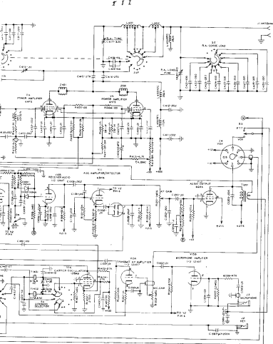
SCHEMATIC DIAGRAM - SWAN MODEL 500 SINGLE SIDEBAND TRANSCEIVER.
