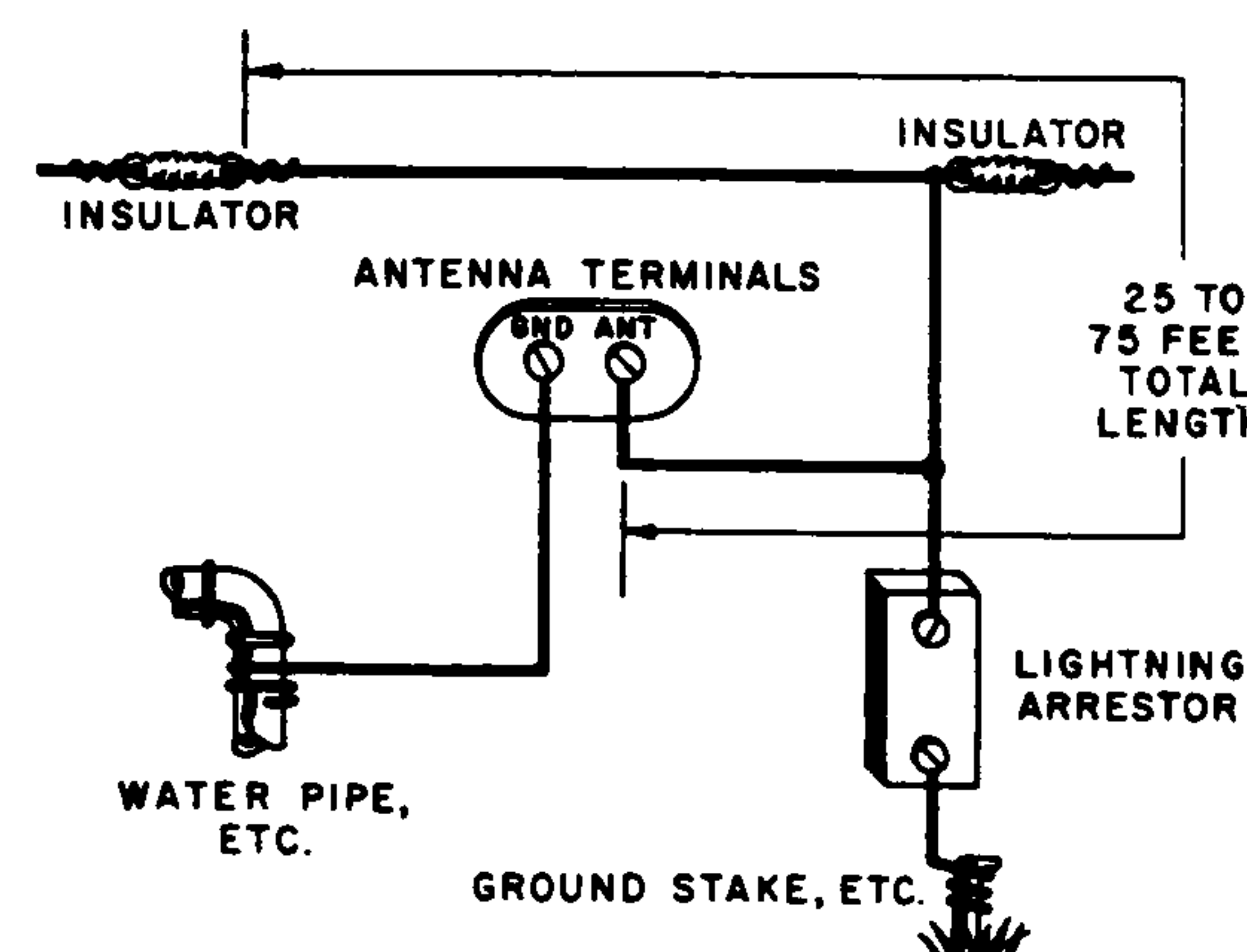
SINGLE WIRE ANTENNA
