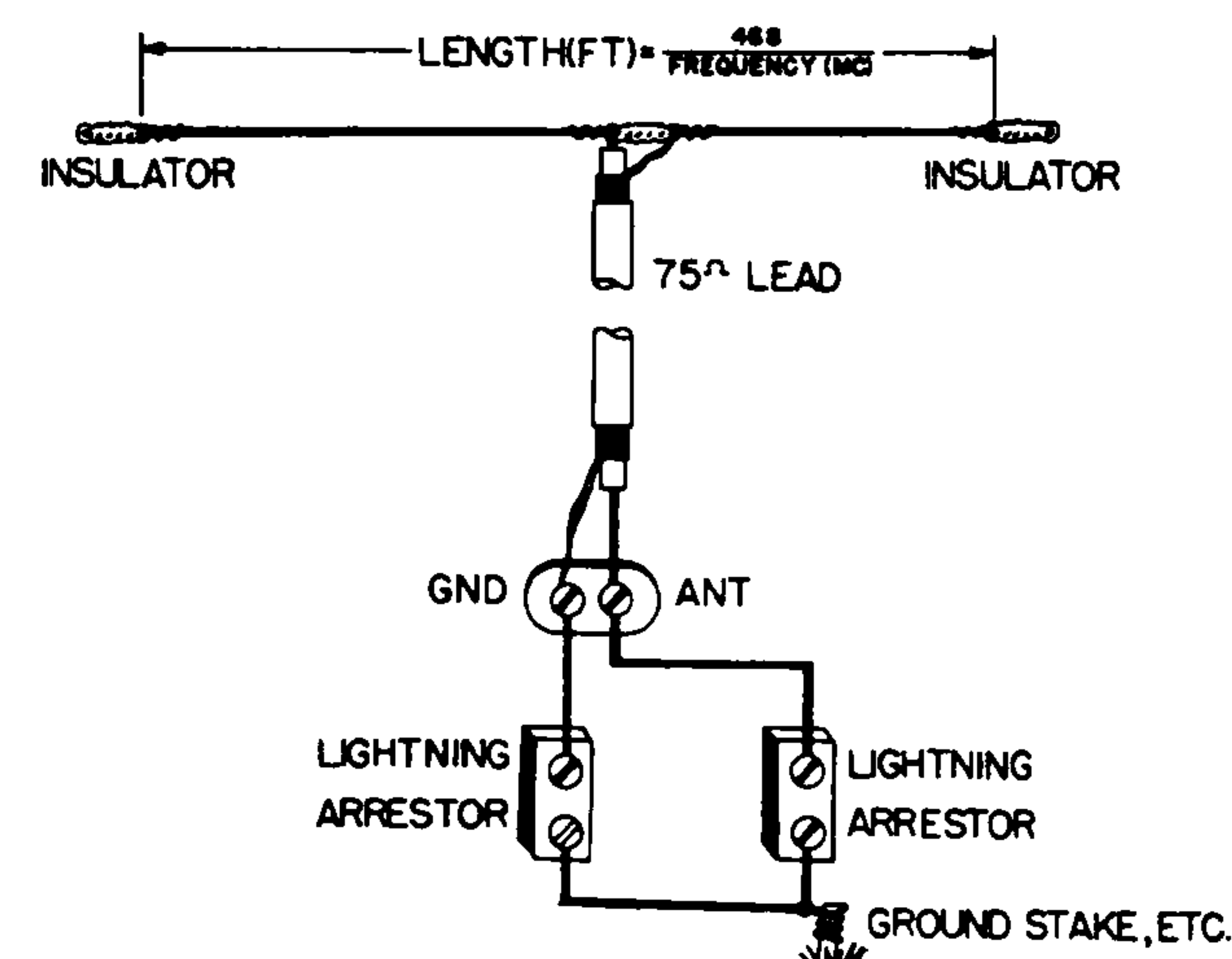
DOUBLET ANTENNA
