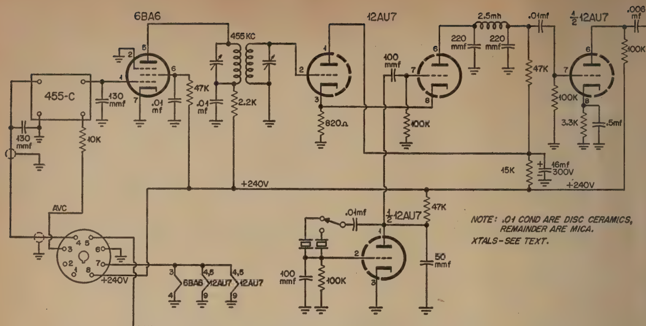
Fig. 1. Schematic of the W6JPU SSB Adapter. Conventional circuitry is used throughout and components are standard. Adjustment of trimmers on the IF transformer is the only tuning required. A crystal oscillator BFO is used to maintain oscillator injection at constant points on the slopes of the Collins Mechanical Filter.
