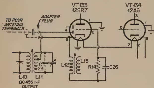
Schematic of adaptor plug.
