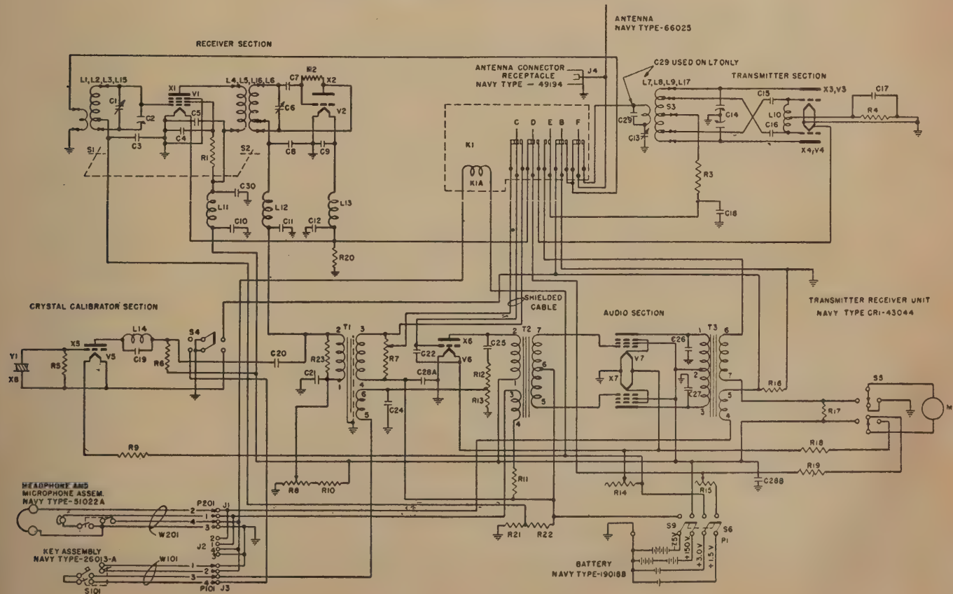
Fig 1. Schematic of unconverted TBY
