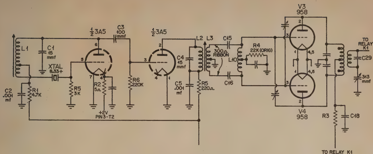
Fig 2. The converted transmitter section of the TBV
