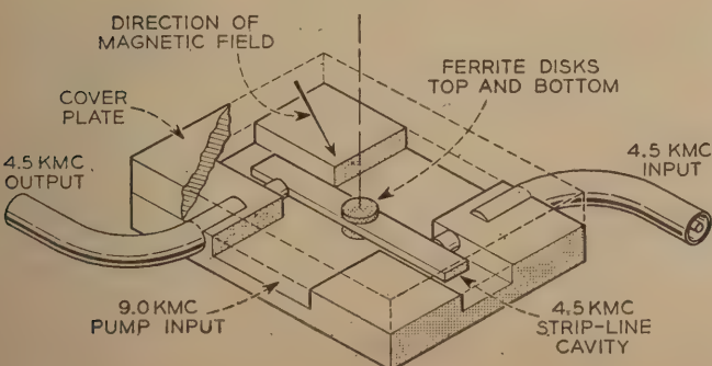
Diagram of an experimental ferrite microwave amplifier which was built at Bell Telephone Laboratories.
