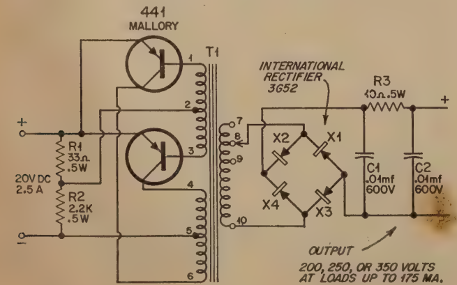
Schematic and load chart.
