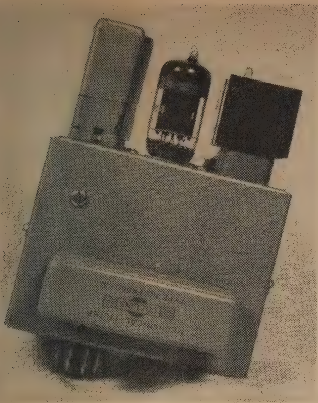
Fig. 3. Top side of the W6JPU SSB Adapter.
