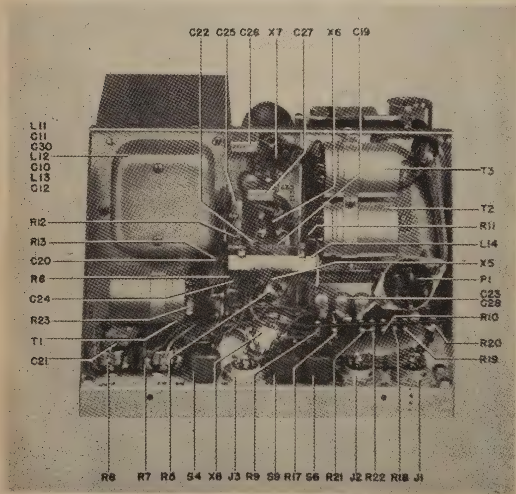
Bottom view of the TBY interior
