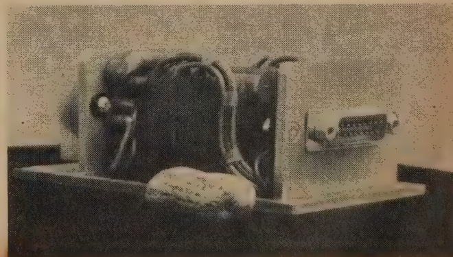
Right-hand and front view. Shows connector, transformer, and transistor at rear. Size is compared to medium-sized peanut.
