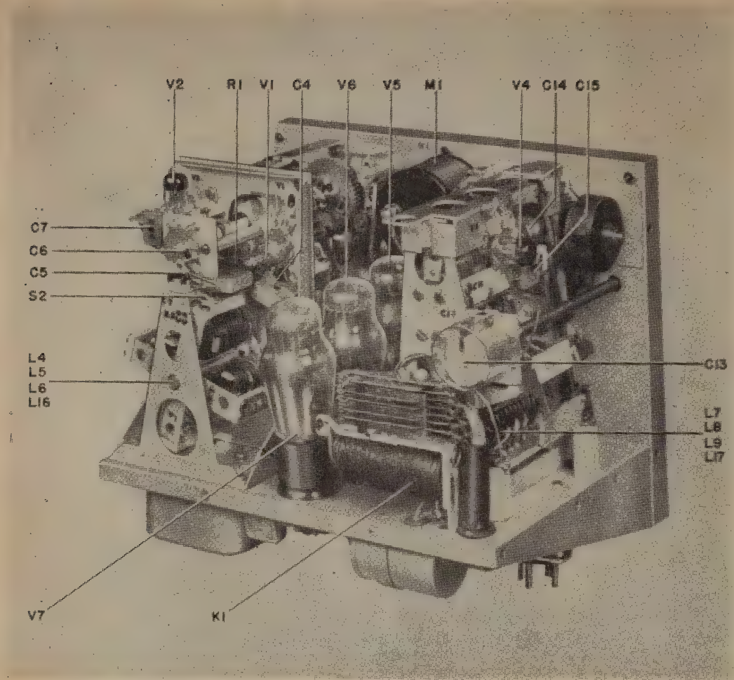
Left Rear view of the TBY interior
