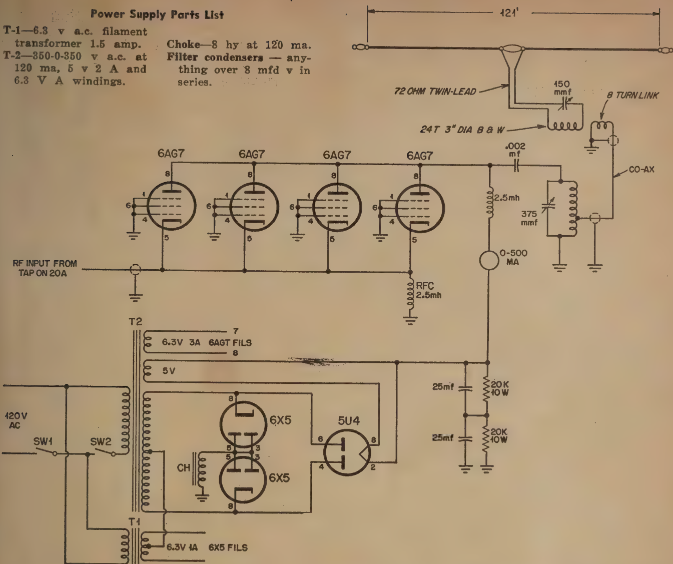
Schematic of unit shown at left.
