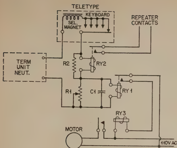
Fig 1—Livingston Autostart Circuit
