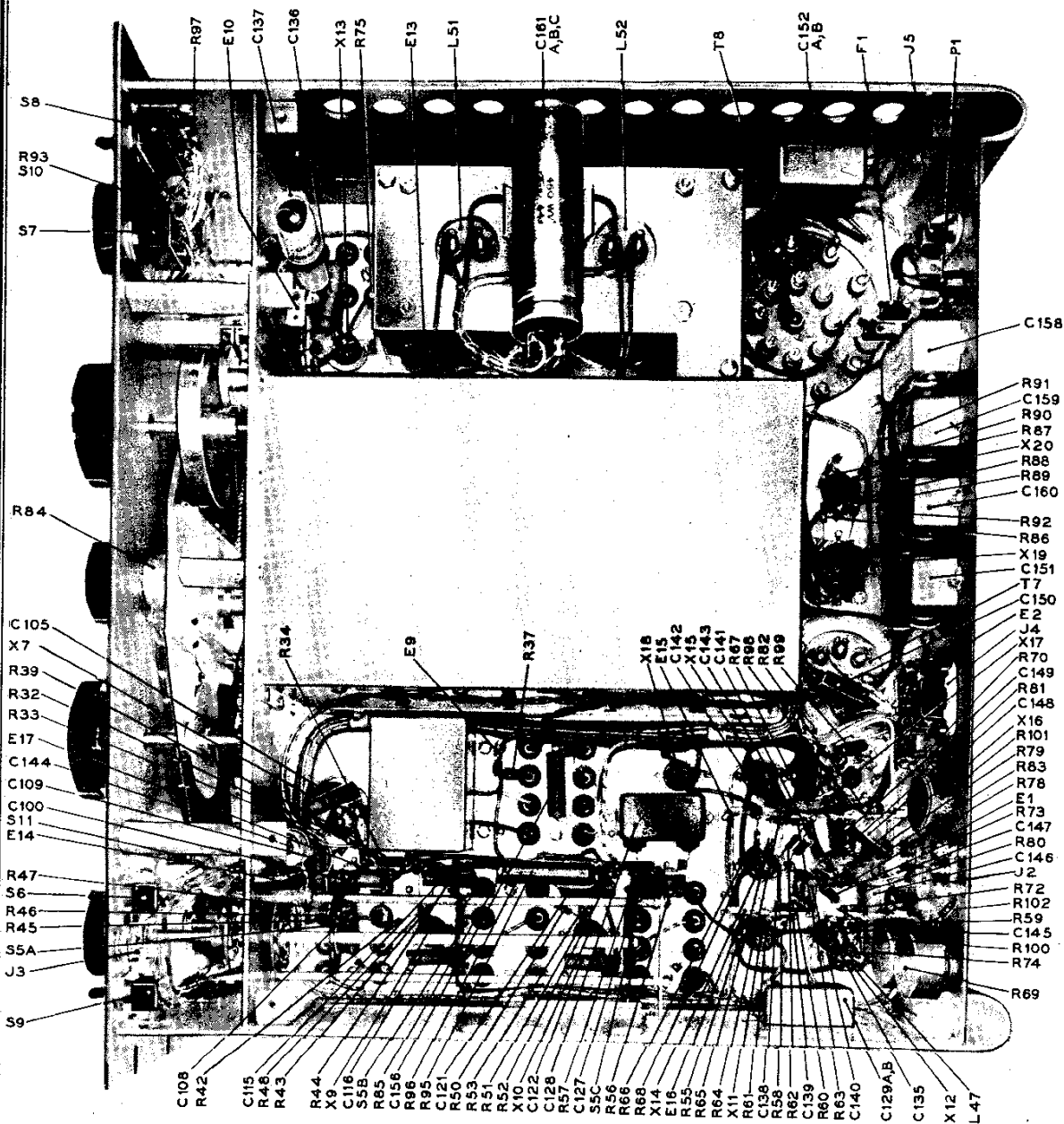
FIG. 9 BOTTOM VIEW OF RECEIVER SP-600-JX
