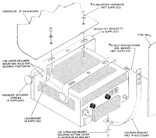
FIGURE 1 MOBILE INSTALLATION
