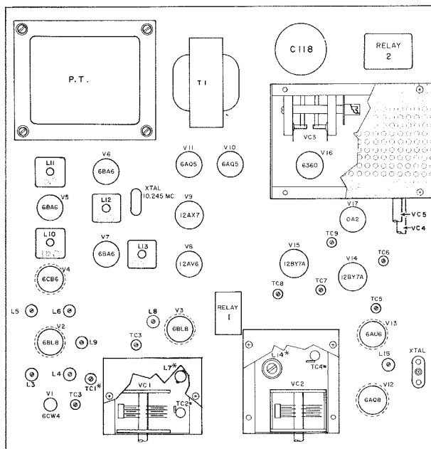
FIGURE 7 TUBE LOCATION AND ALIGNMENT POINTS
