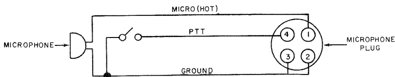
FIGURE 4 MICROPHONE CONNECTIONS
