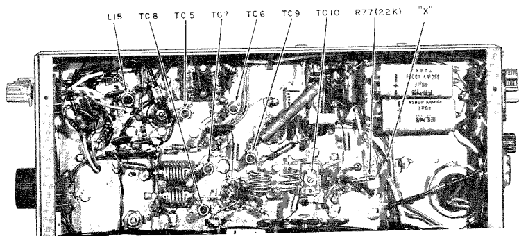
FIGURE 8 TRANSMITTER ALIGNMENT POINTS
