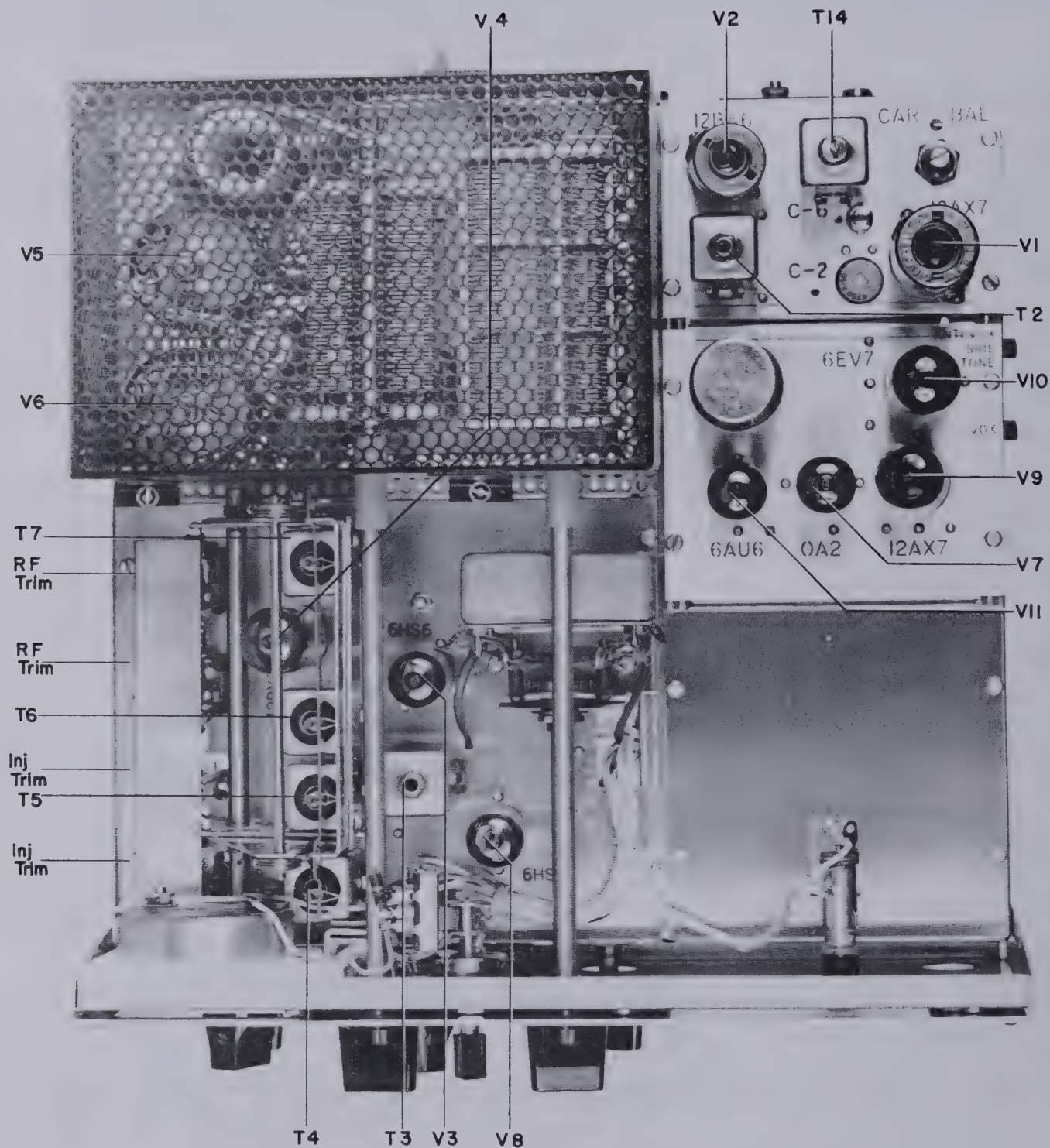
FIGURE 12 TOP VIEW T-4
