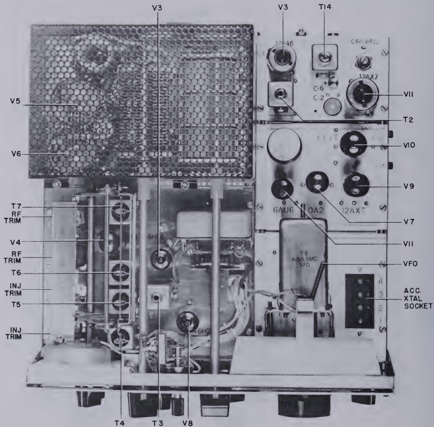
FIGURE 14 TOP VIEW T-4X
