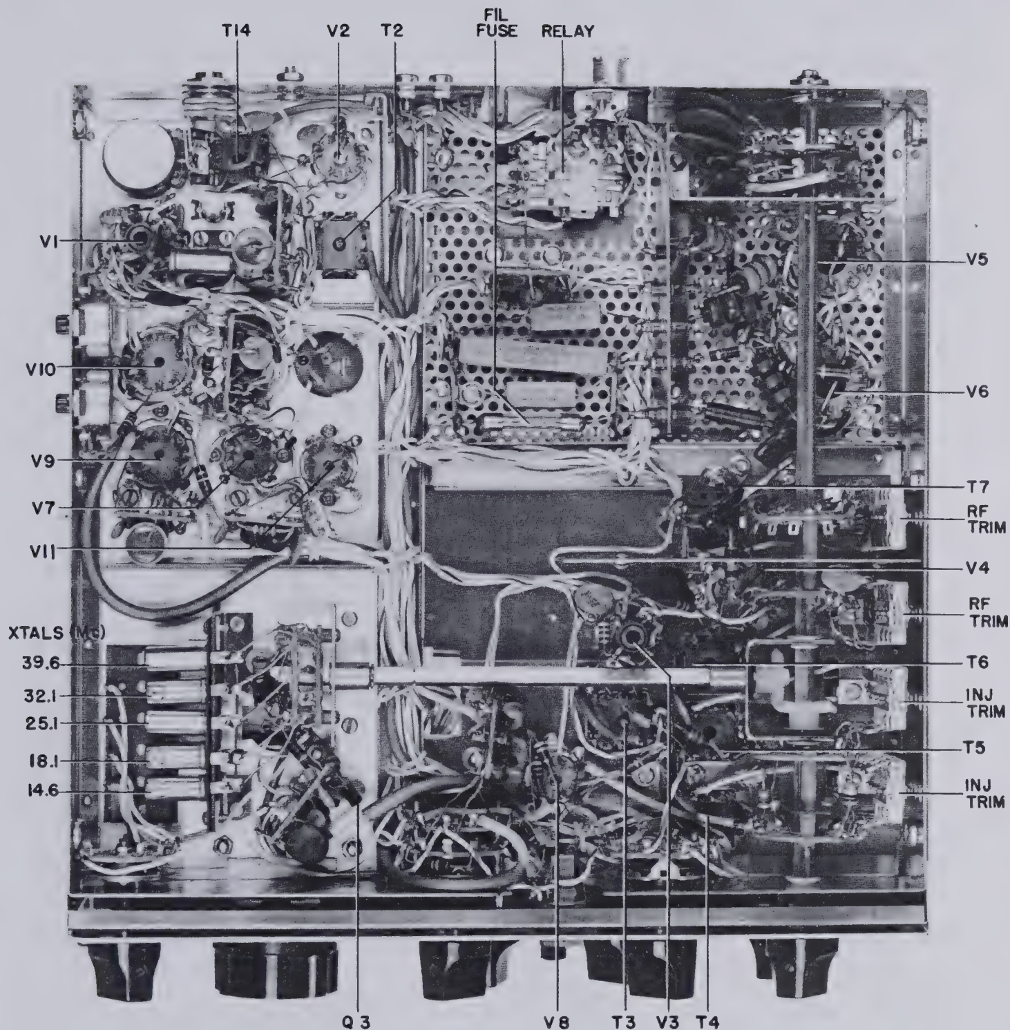
FIGURE 15 BOTTOM VIEW T-4X
