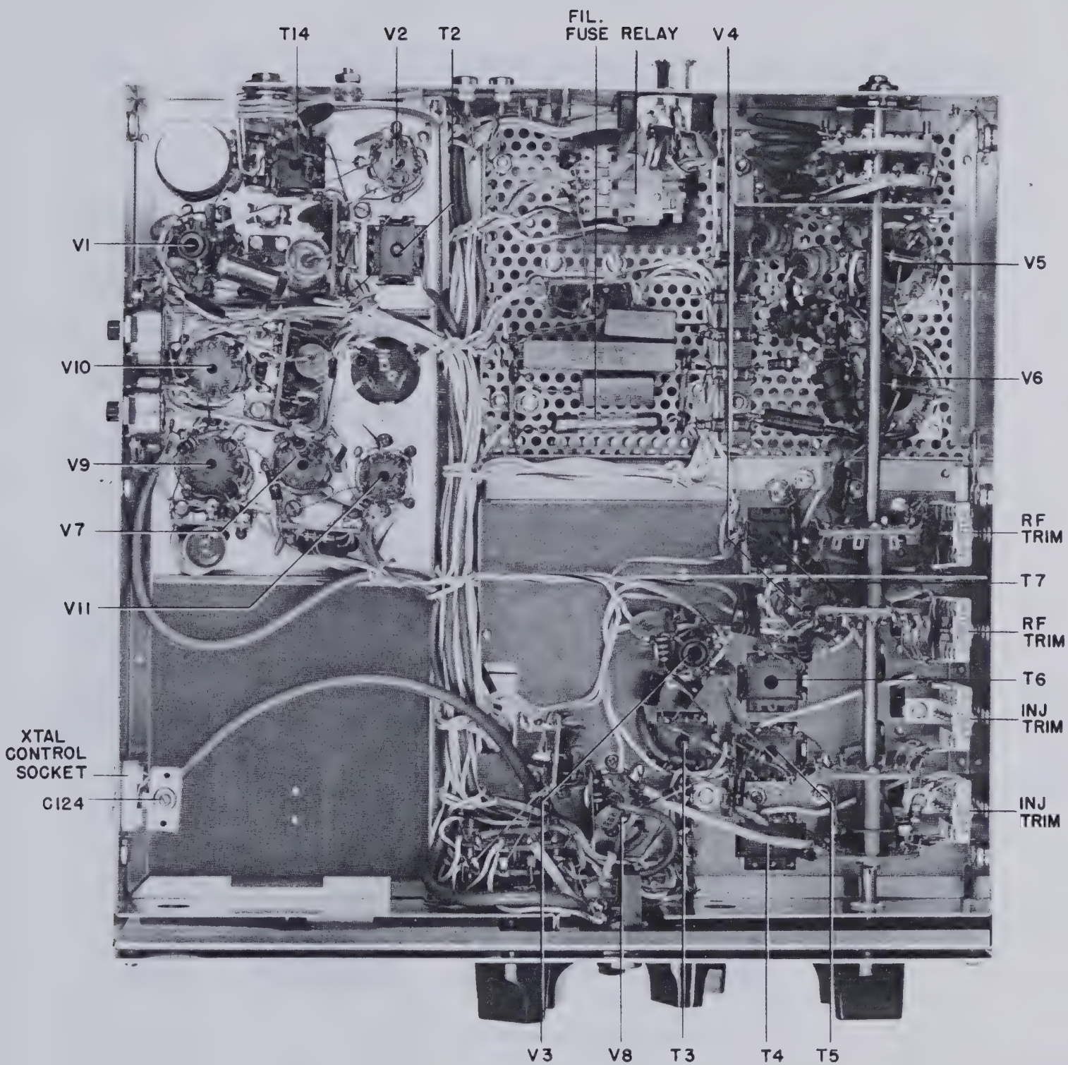
FIGURE 13 BOTTOM VIEW T-4
