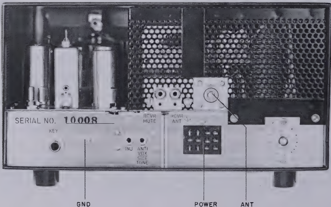
FIGURE 6 REAR VIEW
